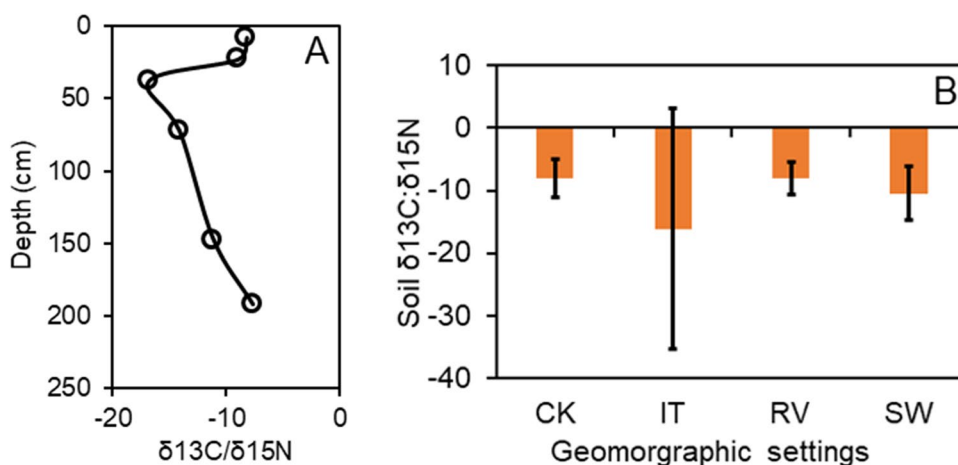
Fig. 10 Mean ratio of \delta^{13}\text{C} to \delta^{15}\text{N} in the mangrove soils (A), and the mean ratio at different settings in the mangrove soils (B) in Rufiji Delta; the bar is standard error ( \pm 1 SD); CK: Creek; IT: Interior; RV: Riverine; SW: Seaward
