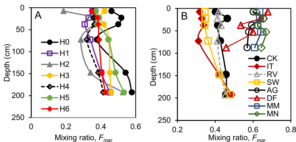
Fig. 11 Mixing ratio of marine OM sources ( F_{\text{mar}} ) for mangrove soils grouped by tree canopy heights, H0 – H6 (A); mixing ratios of marine organic sources for the mangrove and non-mangrove soils grouped by geomorphic settings (B); CK, IT, RV and SW for mangroves, AG, DF, MM and MN for non-mangroves
