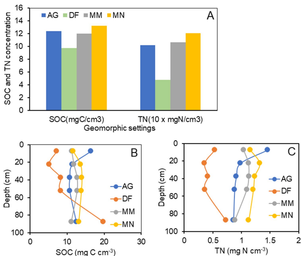
Fig. 7 Overall means of SOC ( \text{mg C cm}^{-3} ) and TN in non-mangrove soils grouped by land types (A), the TN value in panel A is magnified by a factor of 10, the true value should be the value in panel A divided by 10, after that the unit is \text{mg N cm}^{-3} ; AG: agriculture land; DF: dwarf mangrove with very sparse stands; MM: mudflat with recently established mangroves; MN: un-vegetated emergent mudflat; vertical variation in SOC (B) and TN (C) in non-mangrove soils
