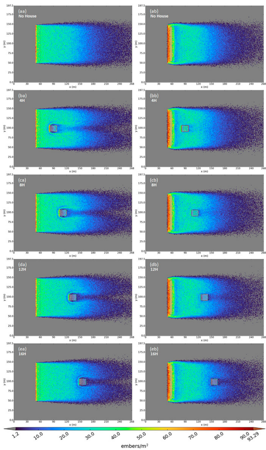
FIGURE 6 Firebrand deposition for the base case experiments. The house is located at various distances downwind with and without the fence present in the flow. The first letter ( A–E ) represents the distance downwind in the flow. The second letter represents the ( A ) absence or ( B ) presence of the fence. The colors represent the deposition per unit area.
