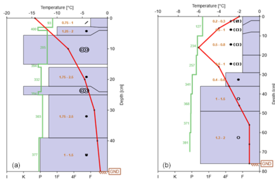
Figure 13. Examples of snowpack profiles measured in Leutasch, AlpSAR campaigns 2B (a) and 3 (b) from snow pit 3.
