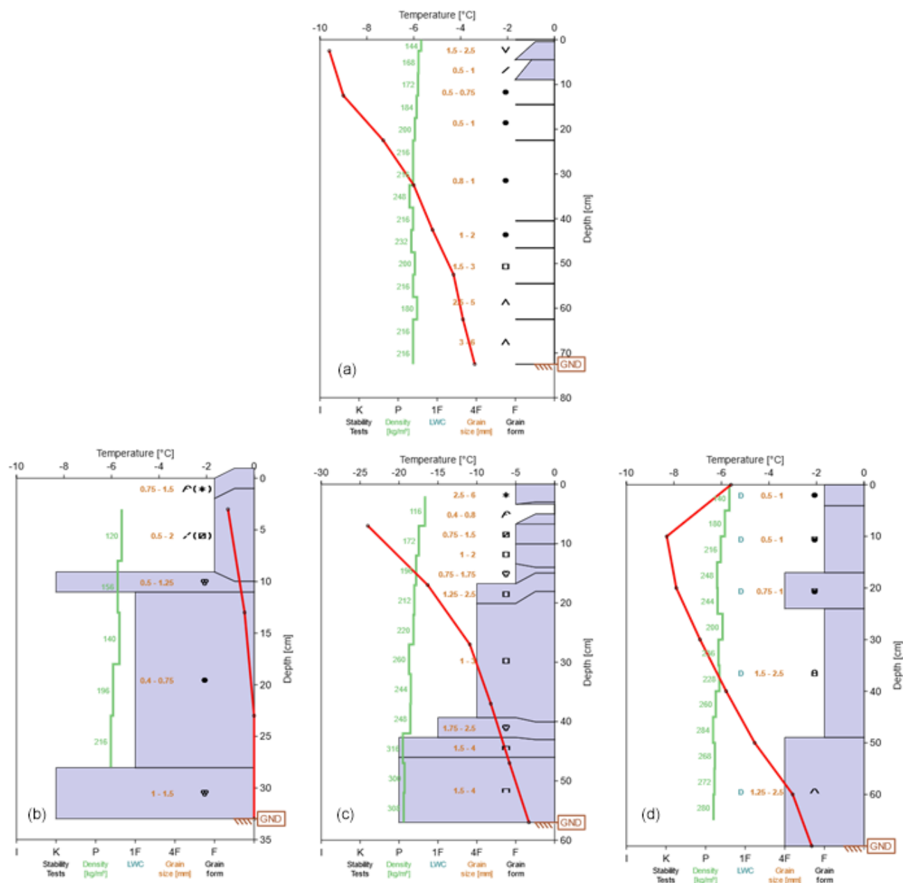
Figure 6. Examples of measured snow profiles in a forest clearing site during NoSREx missions: (a) M00 (17 March 2011) and in the winter of 2011–2012, (b) M01 (19 December 2011), (c) M04 (8 February 2012) and (d) M09 (8 March 2012). Profiles include density (green line), temperature (red line), grain size (minimum–maximum ranges), grain type and hand hardness (vertical bars; K: knife, P: pencil, 1F: one finger, 4F: four fingers and F: fist). Hand hardness was not estimated on 17 March 2011.
