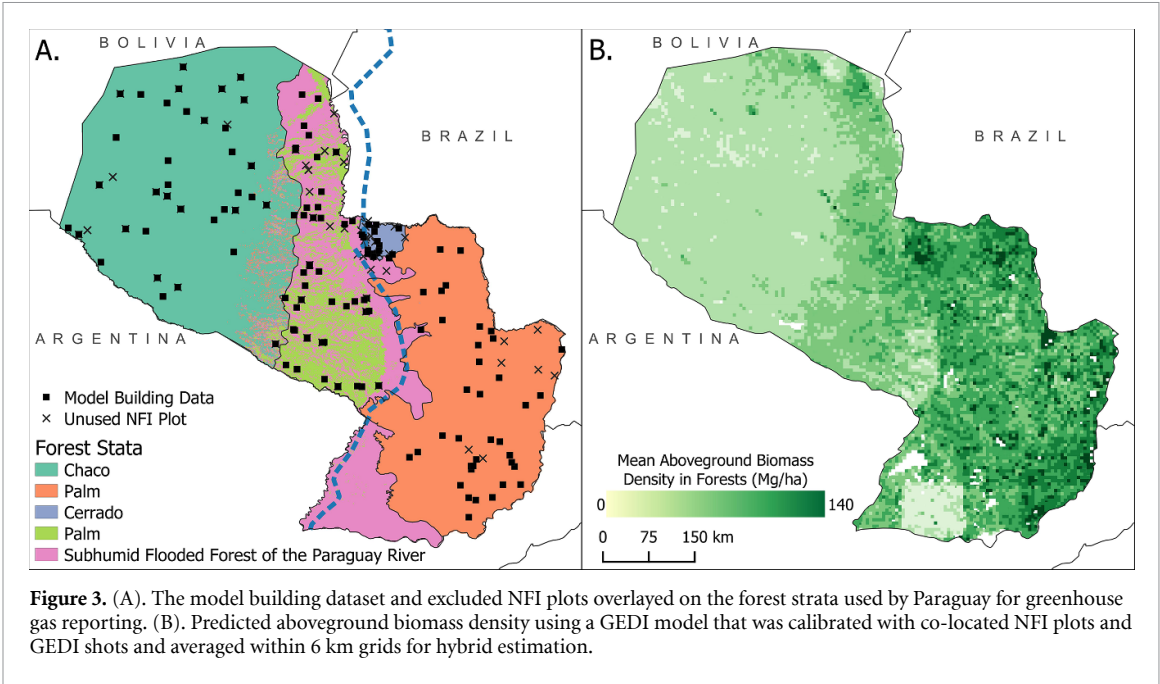
Figure 3. (A). The model building dataset and excluded NFI plots overlaid on the forest strata used by Paraguay for greenhouse gas reporting. (B). Predicted aboveground biomass density using a GEDI model that was calibrated with co-located NFI plots and GEDI shots and averaged within 6 km grids for hybrid estimation.
