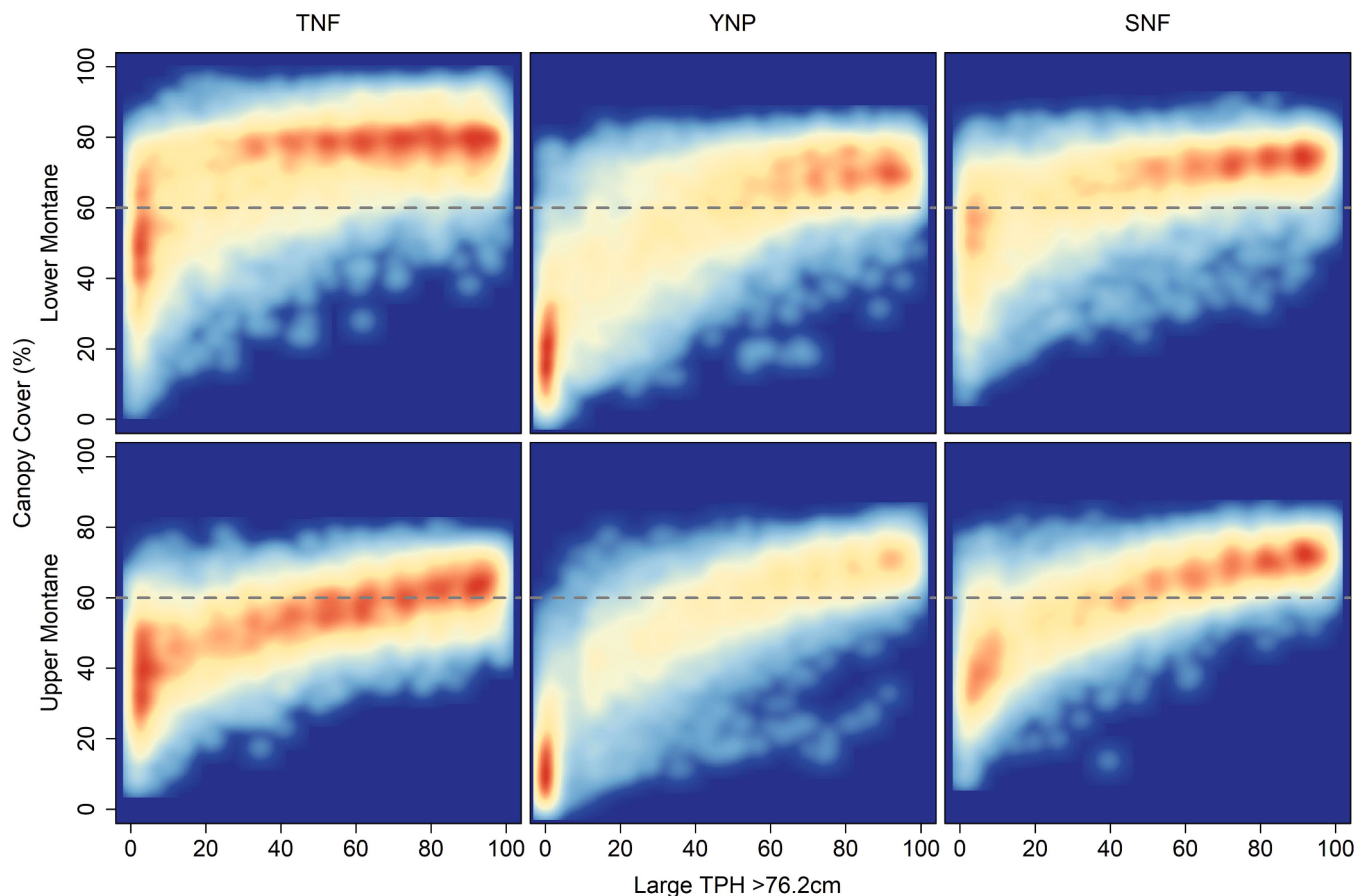
Fig. 5. Relationship of airborne lidar-identified large tree ( >76.2 cm) density per hectare (TPH) to canopy cover calculated from the airborne lidar data for 90 \times 90 m grid cells used in our study. Canopy cover measurements include contributions from trees of all sizes within a grid cell. To create a balanced visualization of all ranges of tree densities, a stratified random sample of tree densities (x axis) was performed in increments of 10 tall trees per hectare, n = 1000 per bin. This allows us to understand how canopy cover varies with density per se, rather than observing the frequency of various density-canopy cover combinations. Without this sampling, high values of large tree densities, which are proportionally rare, would not be visible in the color ramp. Study areas are centered on the Tahoe National Forest (TNF), Yosemite National Park (YNP), and Sierra National Forest (SNF).
