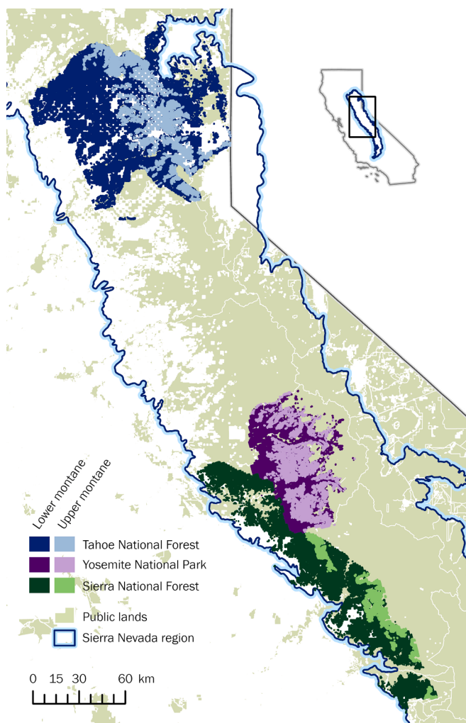
Fig. 1. The Tahoe, Yosemite, and southern Sierra areas used in this study with areas of the low and high montane forest zones shown. Study areas are based on airborne lidar acquisitions that were focused on the Tahoe and Sierra National Forests and Yosemite National Park, but we included additional publicly owned federal, state, and local properties within the footprints of the lidar acquisitions. Online interactive maps available at https://arcg.is/8LfW9 .
