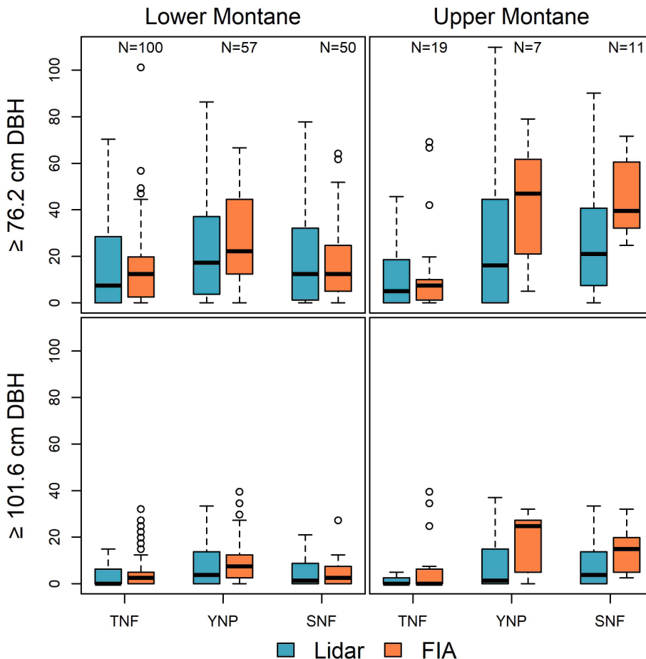
Fig. 2. Large (≥76.2 cm DBH) and very large tree (≥101.6 cm DBH) trees per ha from USDA Forest Service Forest Inventory Analysis (FIA) plots and overstory trees identified from airborne lidar data by forest zone and study area. Numbers of FIA plots used is shown above each pair of bar plots; Table 1 gives sizes of areas examined with airborne lidar data. Tree diameters manually measured for FIA plots and modeled from lidar-identified top of tree heights. Study areas are centered on the Tahoe National Forest (TNF), Yosemite National Park (YNP), and Sierra National Forest (SNF).
