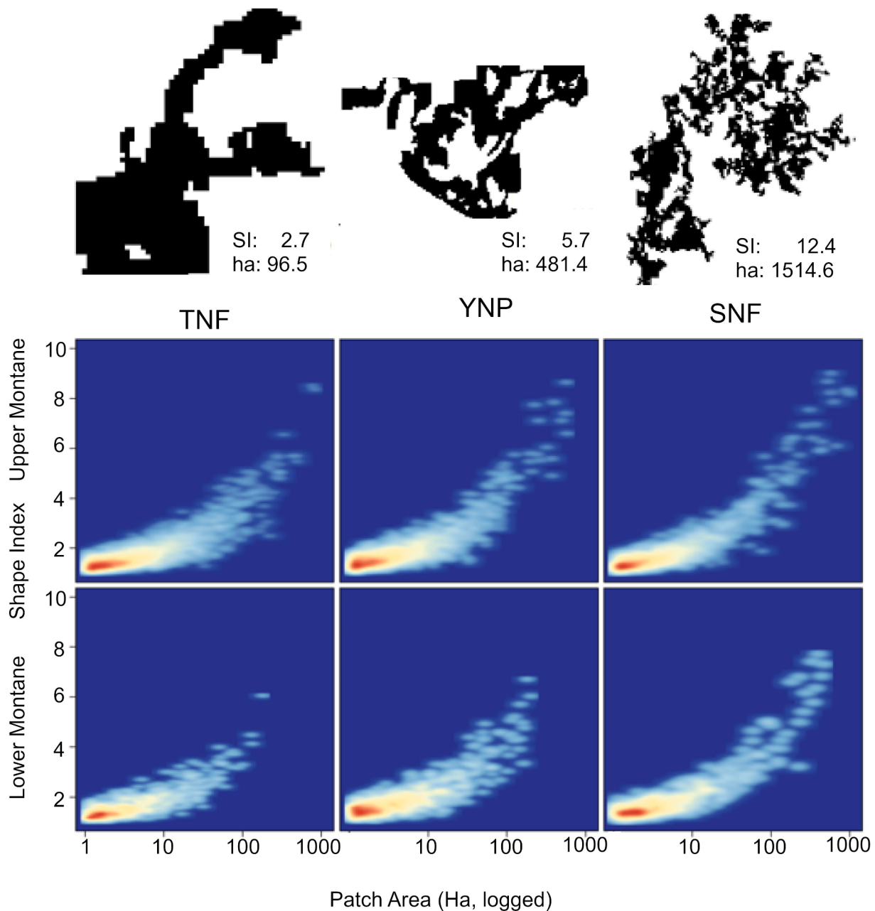
Fig. 7. Complexity of large tree ( \geq 76.2 cm) patches (large tree density > 20 large trees per hectare) by patch size. Top row shows examples of large tree patches for different sizes and shape indices (SI). Lower rows show relationship of patch size to shape index for all large tree patches identified in this study. The shape index calculates a unitless measure of the deviation of a patch's shape from that of a perfect square, which has a value of 1, increasing with patch complexity (unbounded). Study areas are centered on the Tahoe National Forest (TNF), Yosemite National Park (YNP), and Sierra National Forest (SNF).
