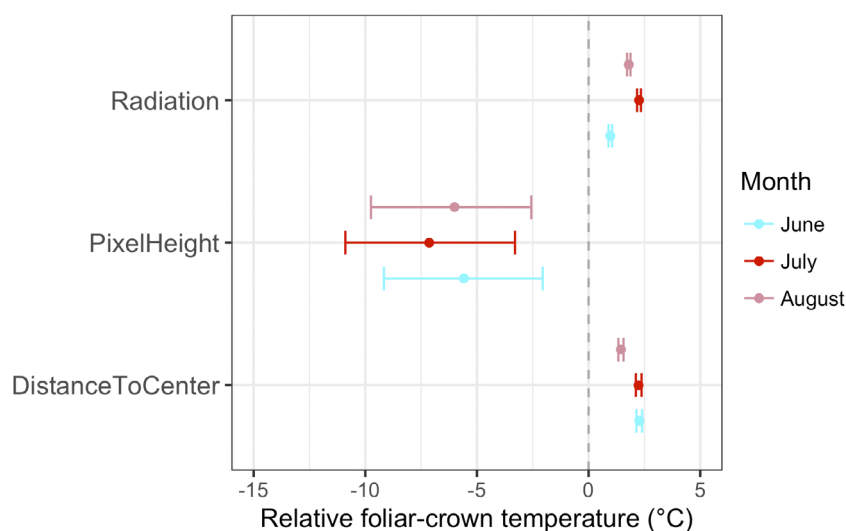
Figure 5. Estimated effects (mean \pm 89% highest posterior density [HPD]) of solar radiation, height above ground (PixelHeight, 1.8 to 2.4-cm pixel resolution), and distance to plant center of each pixel to leaf-level temperature measured by unoccupied aerial systems (UAS).
