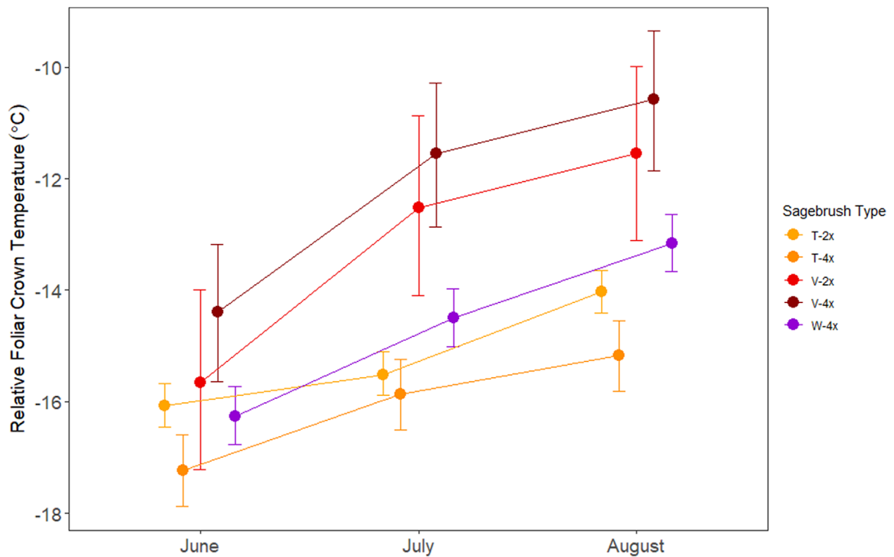
Figure 4. Mean \pm 95% confidence interval relative foliar-crown (plant-level) temperatures ( ^{\circ}\text{C} ) of the different sagebrush types (subspecies and cytotype) by season (5 June, 11 July, 28 August). T = Artemisia tridentata tridentata , basin big sagebrush; V = A. t. vaseyana , mountain big sagebrush; W = A. t. wyomingensis , Wyoming big sagebrush; 2x = diploid; 4x = tetraploid. Temperatures have been centered relative to average ground temperature on each date.
