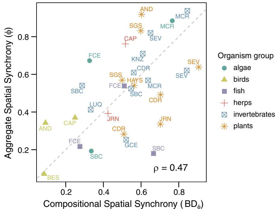
FIGURE 2 The relationship between compositional and aggregate spatial synchrony for all metacommunities (Spearman's \rho = 0.47 ). Metacommunities above the 1:1 line had a smaller reduction in aggregate than compositional variability from local to regional scales, while those below the 1:1 line had a relatively greater reduction in aggregate than compositional variability.
