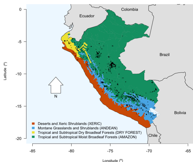
Figure 2. Map of the Peruvian ecoregions considered in this study, with 2001–2020 GlobFire centroids of large, multi-day fires overlaid.
