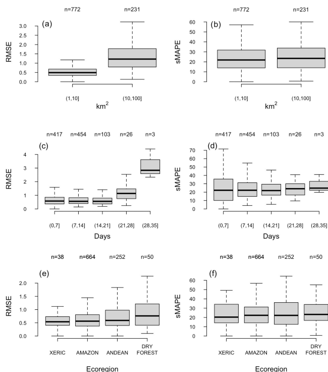
Figure 5. Boxplots of root-mean square error estimates calculated from best-fit difference equation predictions and GlobFire observations. Root-mean square error estimates are disaggregated by size, duration, and ecoregion. Sample size is reported above the boxplots, and outliers have been removed for visualization purposes.
