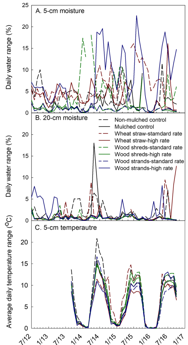
Fig. 2. Monthly average daily water range at (A) 5-cm and (B) 20-cm depth, and (C) daily temperature range at 5-cm depth measured as the difference between daily maximum and minimum percent volumetric water content or soil temperature, respectively. Mulch application rate treatments were Burned Area Emergency Response (BAER) standard (dashed) and 150% of BAER standard by weight (high rate, solid). Mulches were applied in July 2012. Due to periodic logger failure, statistical analysis included only treatments and months with data available from at least three replicate plots (Supplement B). Data presented and analyzed on the original scale.
