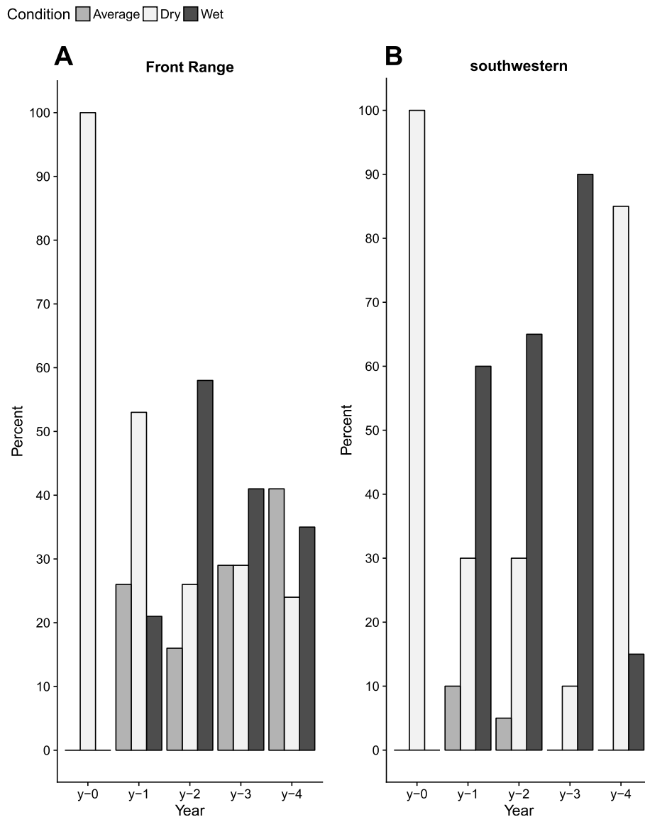
Fig. 11 Relationship between fire year and antecedent precipitation conditions from 12 fire history studies in ponderosa pine ( Pinus ponderosa ) ecosystems for two geographic regions, (A) Front Range ( n = 19 ) and (B) southwestern ( n = 20 ) in Colorado, USA, used in the fire regime meta-analysis of 2017. Y-axis represents the percent of all observations in each of three precipitation conditions: average precipitation, dry (below average), and wet (above average). Precipitation condition is derived from a combination of climate indices including, Palmer Drought Severity, tree-ring growth, NINO3 sea surface temperature, and others. X-axis represents the year relative to fire year (y-0 is fire year, y-1 is year before fire year, and so on)
