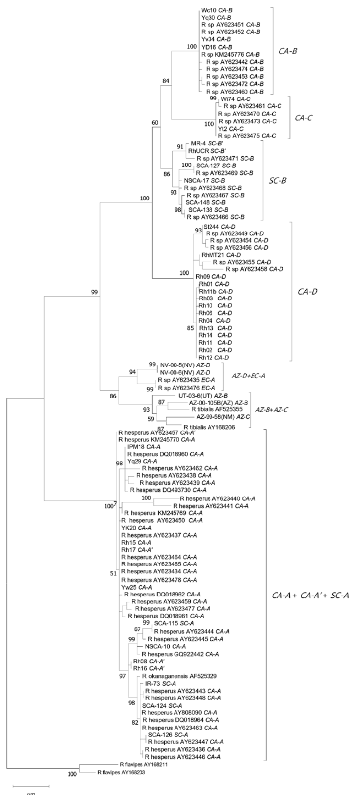
Fig. 1. Maximum likelihood phylogeny of Reticulitermes based on partial COII gene (680 bp). Numbers above branches indicate ultrafast bootstrap values calculated by IQ-TREE. The tip labels indicate the sample identity as labeled in GenBank, followed by the cuticular hydrocarbon (CHC) type in italics. For samples not collected from California, the location is denoted by state abbreviation in brackets following the sample identity.
