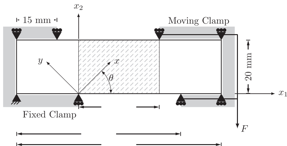
FIGURE 3 Schematic of unnotched Iosipescu geometry. Centre, shaded region indicates grid inspection area. Angle \theta represents ring orientation and is aligned with the axes of material orthotropy, x, y . Model was 2.3 mm thick. F is applied force
