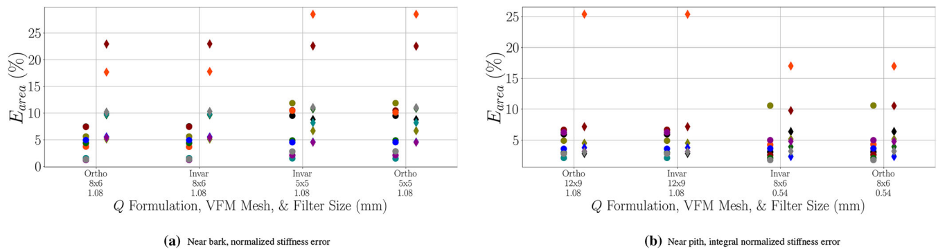
FIGURE 16 Integral normalized stiffness error at \theta = 35^\circ for different Q formulations, VFM meshes and Savitsky–Golay size filters. Figure 15 contains the legend
