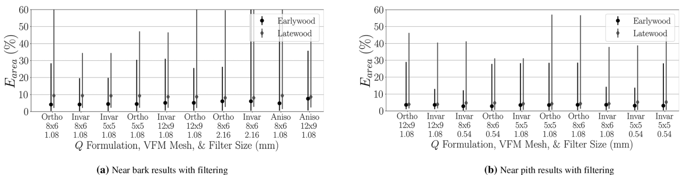
FIGURE 13 Comparison of E_{area} at \theta = 35 for different Q formulations, VFM meshes (Figure 5) and Savitzky–Golay size filters (mm). Markers represent median value and error bars represent data range. Ortho, orthotropic; Invar, invariant; Aniso, anisotropic. EW and LW data are offset from each for visualization
