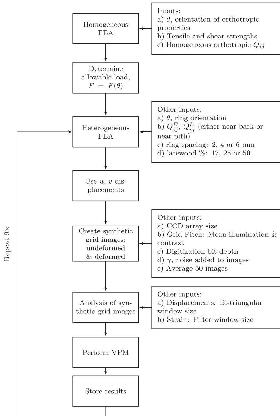
FIGURE 6 Flowchart of simulation procedure
