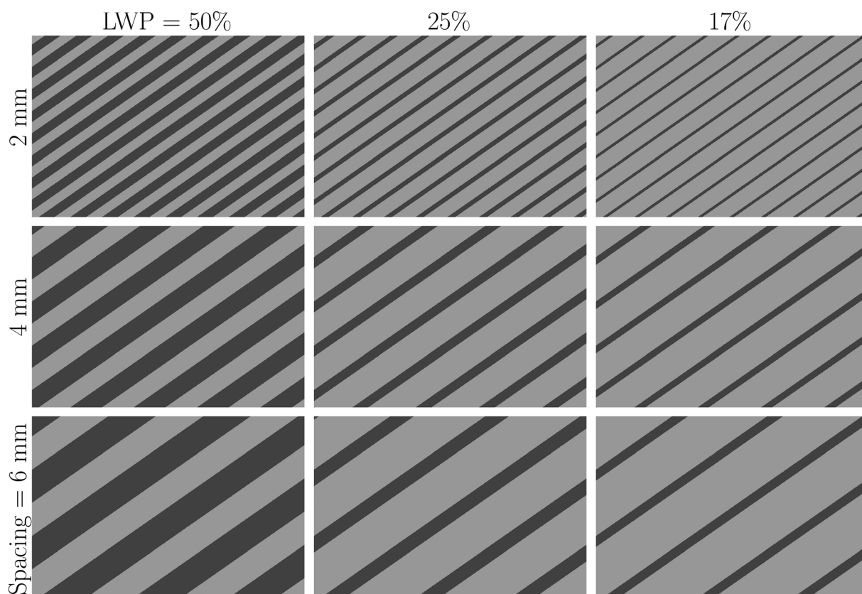
FIGURE 1 Example ring spacing and LW/EW ratios for \theta = 35^\circ . Only centre examination region is shown and has dimensions 30 mm wide × 20 mm high
