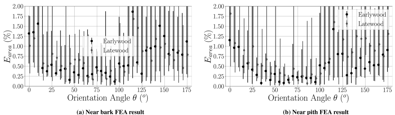
FIGURE 10 E_{area} for FEA data. Markers are at the median value and error bars denote data range. EW and LW data are offset from each for visualization
