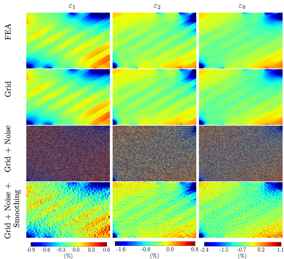
FIGURE 8 Strains produced during simulation processes. In this example, \theta = 30^\circ , ring spacing = 4 mm, and LWP = 50%. Smoothing window for final row was 0.54 × 0.54 mm
