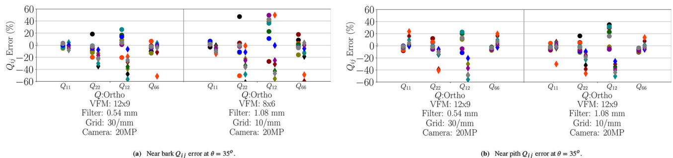
FIGURE 17 Individual Q_{ij} error at \theta = 35^\circ ; ◆ = LW, • = EW. Figure 15 contains the legend
