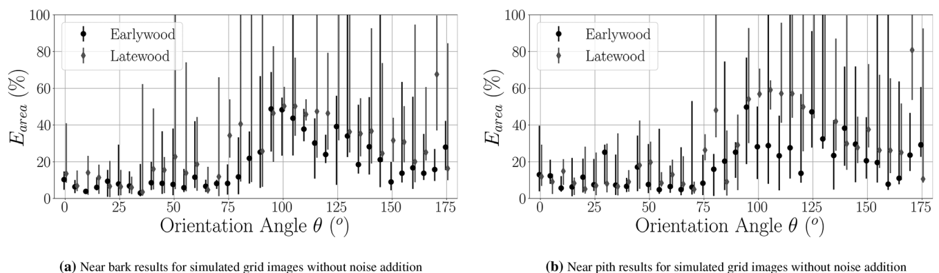
FIGURE 11 E_{area} using simulated grid images with no noise. Markers represent median value and error bars represent data range. EW and LW data are offset from each for visualization
