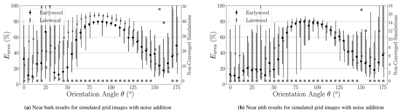
FIGURE 12 E_{area} for grid images with noise addition. Markers represent median value and error bars represent data range. Second (right) vertical axis denotes simulations without convergence. EW and LW data are offset from each for visualization
