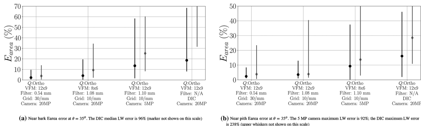
FIGURE 14 E_{area} error at \theta = 35^\circ . Markers represent median value and error bars represent data range. \blacklozenge = LW, \bullet = EW
