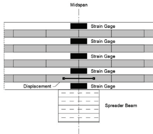
Figure 8 Schematic of Strain Gages at Panel Edge
