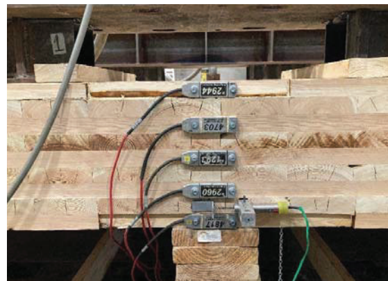
Figure 9 Strain Gages at Panel Edge
