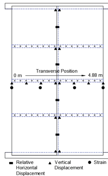
Figure 7 Deflection and Strain Gage Placement
