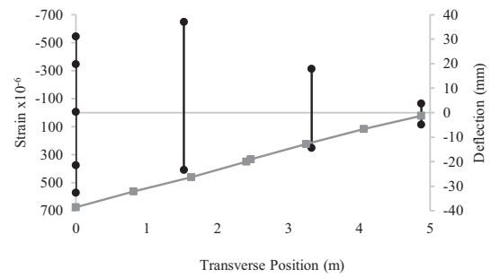
Figure 14 Strain and Deflection at Max Load for Load Case 1
