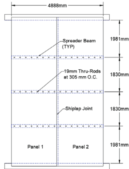
Figure 3 Plan View of Longitudinal Deck Panel Configuration
