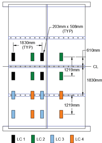
Figure 6 Location of Rear-Axle Tandems for each Load Case
