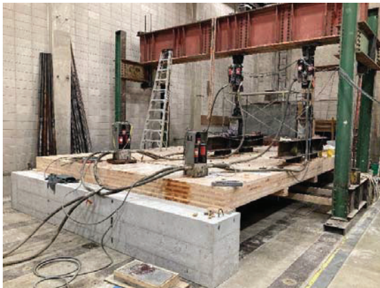
Figure 2 Longitudinal Panel Test Configuration
