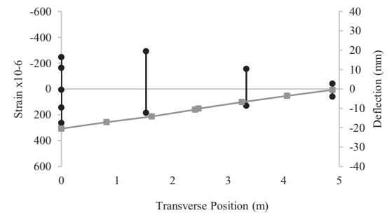
Figure 16 Strain and Deflection at Max Load for Load Case 3
