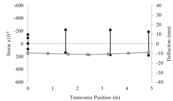
Figure 17 Strain and Deflection at Max Load for Load Case 4
