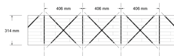
Figure 5 Screw Pattern along Longitudinal Panel Shiplap Joint
