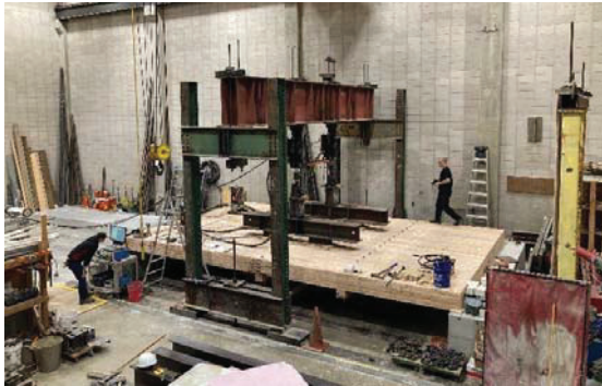
Figure 11 Load Case 2
