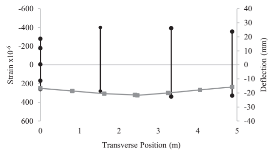
Figure 15 Strain and Deflection at Max Load for Load Case 2
