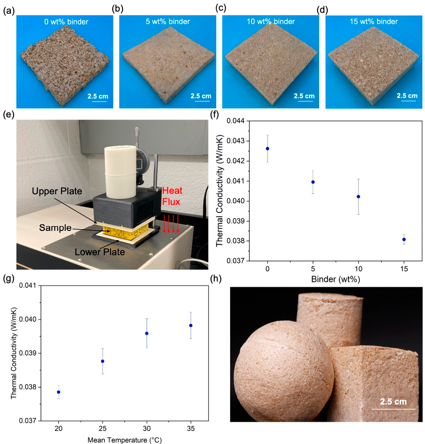
Figure 4. Thermal insulation performance. Delignified wood chip foam samples with varied CMC binder content, including (a) 0 wt.% binder, (b) 5 wt.% binder, (c) 10 wt.% binder, and (d) 15 wt.% binder. (e) HFM-25 apparatus. (f) Thermal conductivity of delignified wood chip foam versus CMC binder content. (g) Thermal conductivity of 15 wt.% CMC binder delignified wood chip foam versus mean temperature. (h) Wood chip foams with different shapes.
