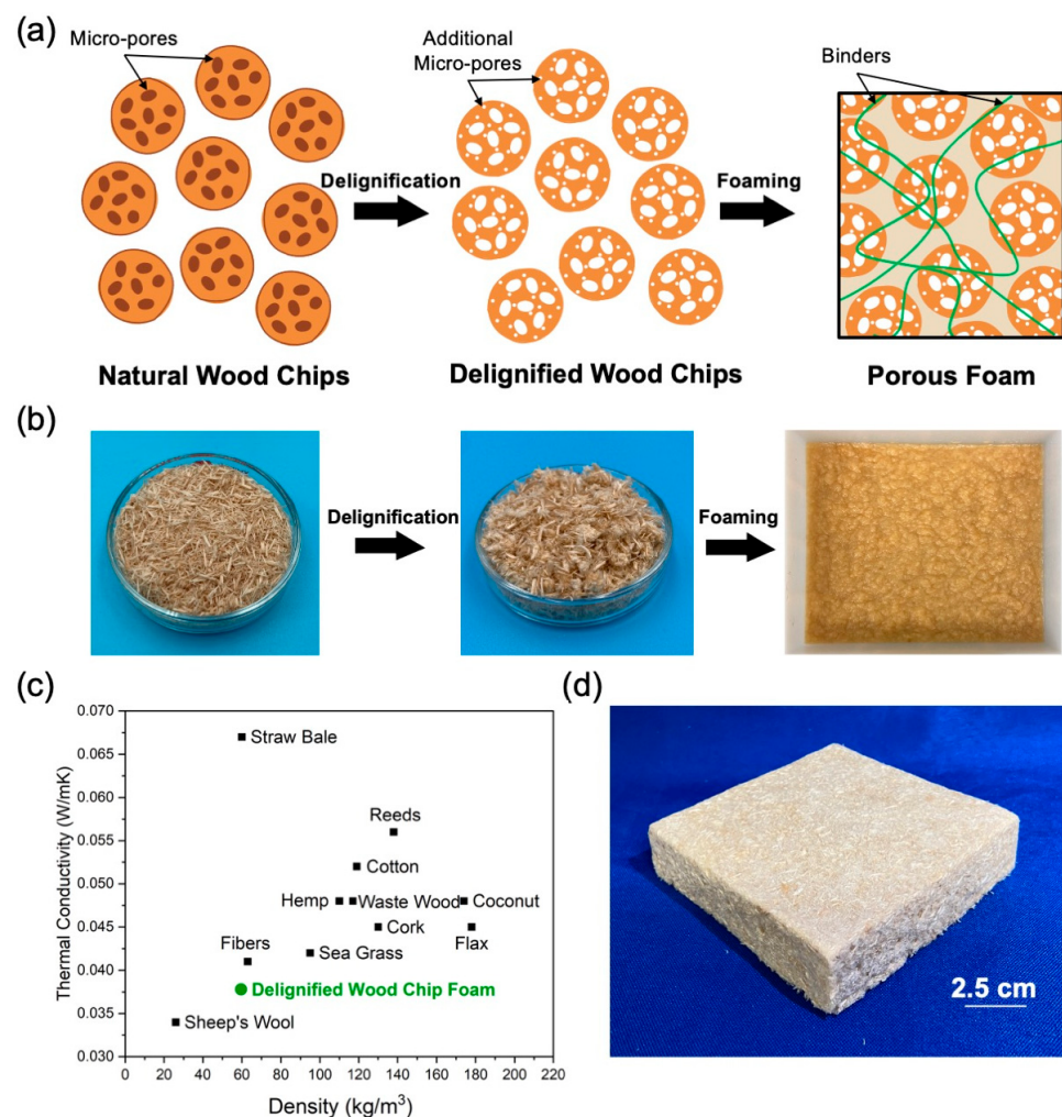
Figure 1. Fabrication process. (a) Detailed schematic and (b) photographs of the foaming fabrication process. (c) Thermal conductivity comparison of various bio-based thermal insulation materials. (d) Newly fabricated porous foam from delignified poplar wood chips.
