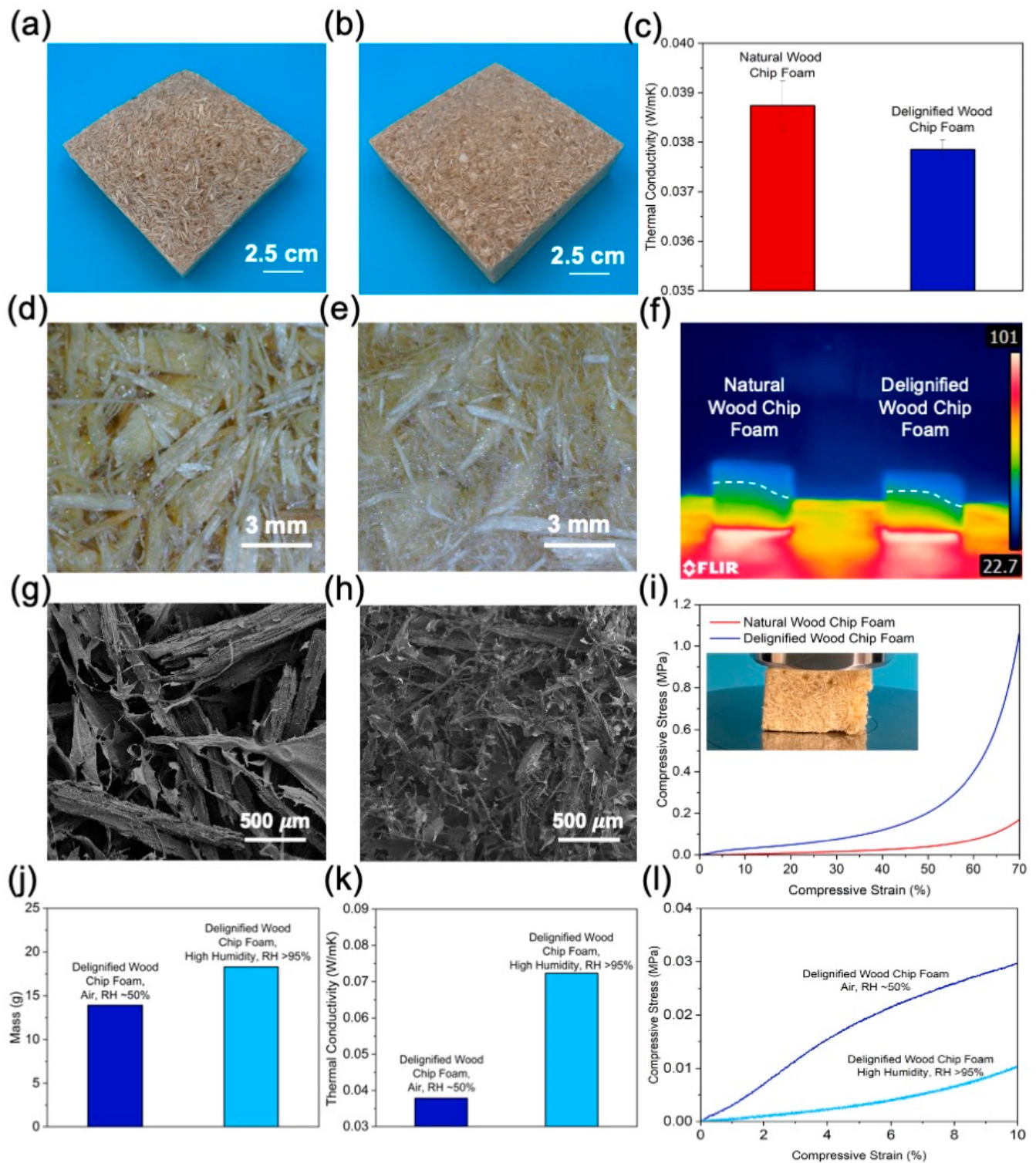
Figure 3. Performance properties of 15 wt.% CMC binder wood chip foams. (a) Natural and (b) delignified foams. (c) Thermal conductivities of the natural and delignified foams. Optical microscope images of the (d) natural and (e) delignified foams. (f) Infrared camera image. SEM images of the (g) natural and (h) delignified foams. (i) Compressive strength graph. Influence of moisture of the 15 wt.% CMC binder delignified wood chip foam on (j) mass, (k) thermal conductivity, and (l) compressive strength.
