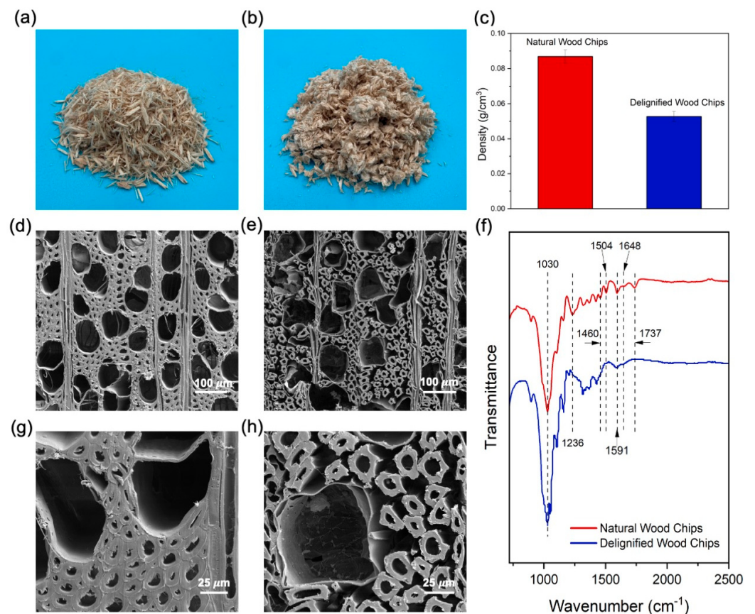
Figure 2. Structural and compositional characterization. (a) Natural and (b) delignified wood chips. (c) Density comparison of natural and delignified wood chips. SEM images of (d) natural and (e) delignified wood chips. (f) FTIR spectra. Magnified SEM images of (g) natural and (h) delignified wood chips.
