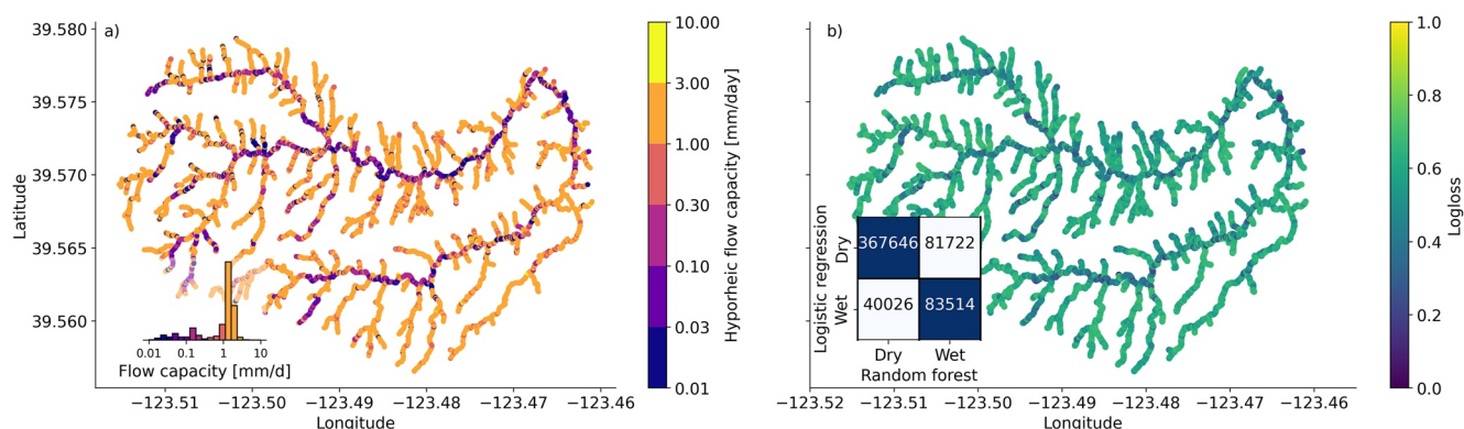
Figure 6. (a) Map of inferred hyporheic flow capacity shows decreased area-normalized ( L T^{-1} units) flow capacity at higher drainage areas (main channel stems). Inset shows histogram of flow capacities. (b) Fit quality information for flow capacity logistic regressions (see Methods), including a map of log loss and (inset) a confusion matrix of logistic regression predictions compared to the random forest predictions to which they are fit. Fit quality is lower at higher logloss.
