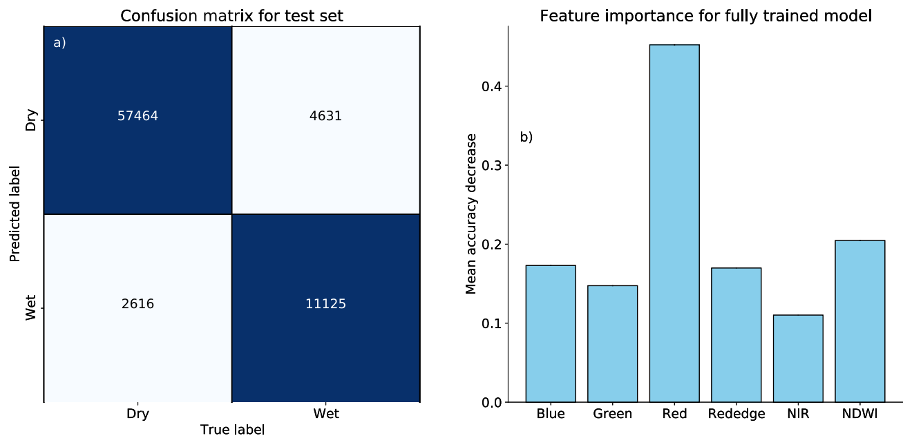
Figure 3. (a) Confusion matrix illustrating prediction accuracy of random forest classifier model (trained on 75% of original data) on test data (25% with-held data points). (b) Permutation feature importance for features in model trained on full training data set.
