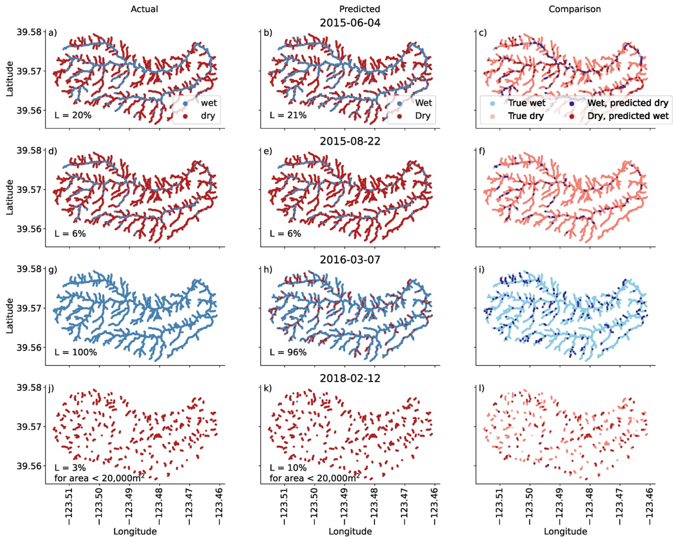
Figure 4. Visual representation of model performance on the four primary training dates. In each subplot, L expressed the extent of active channel as a percent of total channel length (wet plus dry). The top rows are the surveyed dates in summer 2015. The third row represents a fully wetted network during a wet season peak flow event, and the bottom (drone survey data) represents an image during the wet season when many small channels are nevertheless dry. The fourth row does not illustrate continuous networks because we only have suitable training data for contributing areas less than 20,000 m 2 on this particular date.
