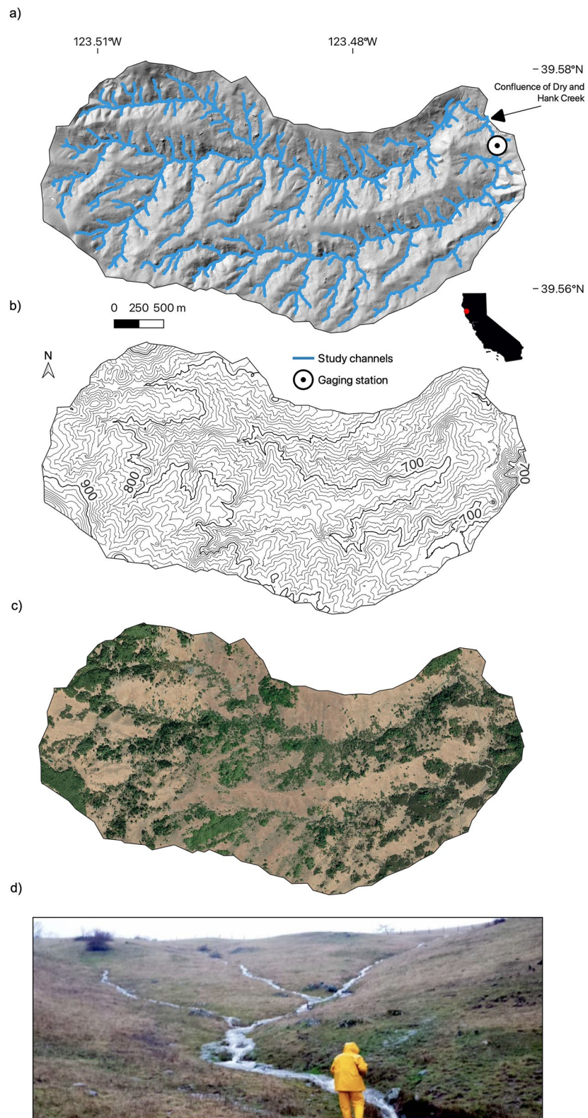
Figure 1. Hillshade of adjacent study catchments with study channels and gauging station location (a) and topographic map with 10 m spaced elevation contours (b, elevations labeled in meters) both derived from a Lidar digital elevation model. Panel (c) shows aerial imagery (bottom, Esri “World Imagery,” accessed 27 September 2022). Panel (d) is a photograph taken of a Dry Creek sub-catchment during a high flow event, from Hahm et al. (2019).
