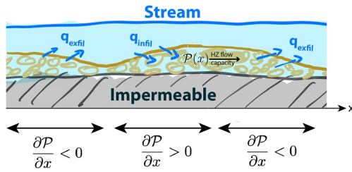
Figure 2. Simplified stream profile illustrating drivers of hyporheic exchange flows. Where volumetric flow capacity ( P ) in the HZ decreases in the downstream ( x ) direction ( \frac{\partial P}{\partial x} < 0 ), there will be hyporheic exfiltration into the stream. Where flow capacity increases with x , there will be infiltration from the stream into the HZ.
