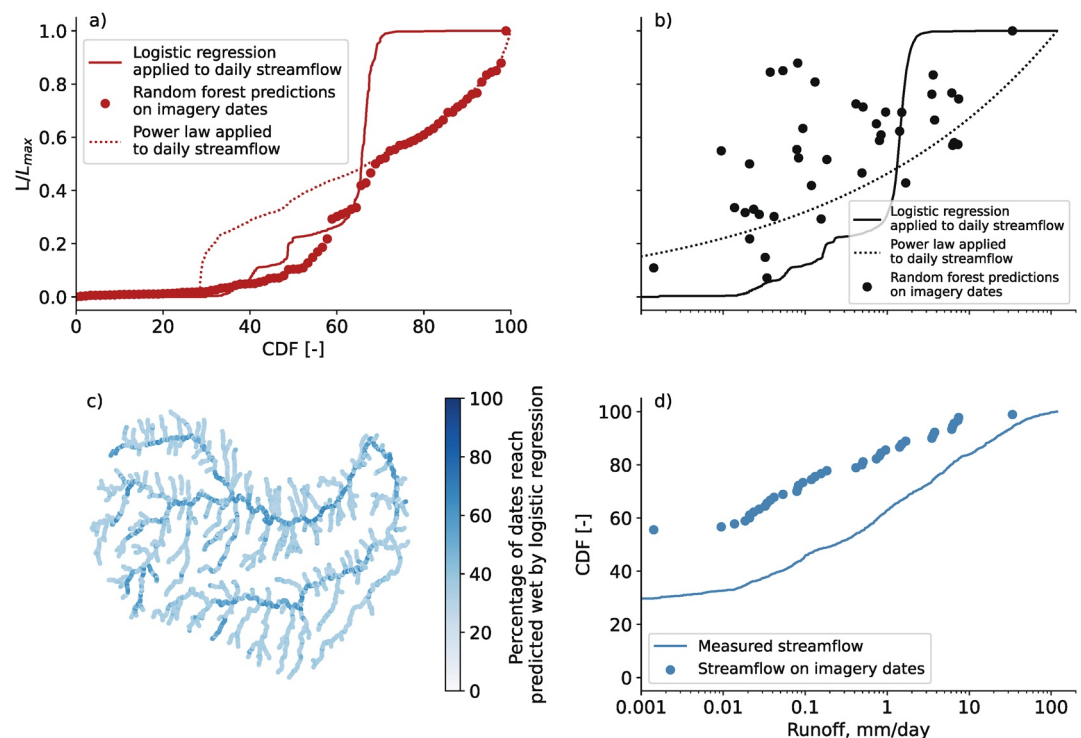
Figure 9. (a) Empirical cumulative distribution function (CDF) of wetted channel length from three methods: random forest-estimated wetted network length on imagery dates (scatter points), power law model trained on random forest results aggregated to total network length applied to all daily streamflow (dotted line), and logistic regression trained at each reach on random forest results applied to all daily streamflow (solid line). (b) Relationship between runoff and wetted channel length as estimated by each of the three methods. (c) Map of reach persistence based on logistic regression applied to all daily streamflow. (d) CDF of runoff using (solid line) all streamflow data during the study period and (scatter points) only streamflow on imagery dates. The CDF does not go to zero at the lowest non-zero flows because flow is zero (and thus not plot-able on a log scale) for a large fraction (roughly 30%) of the year.
