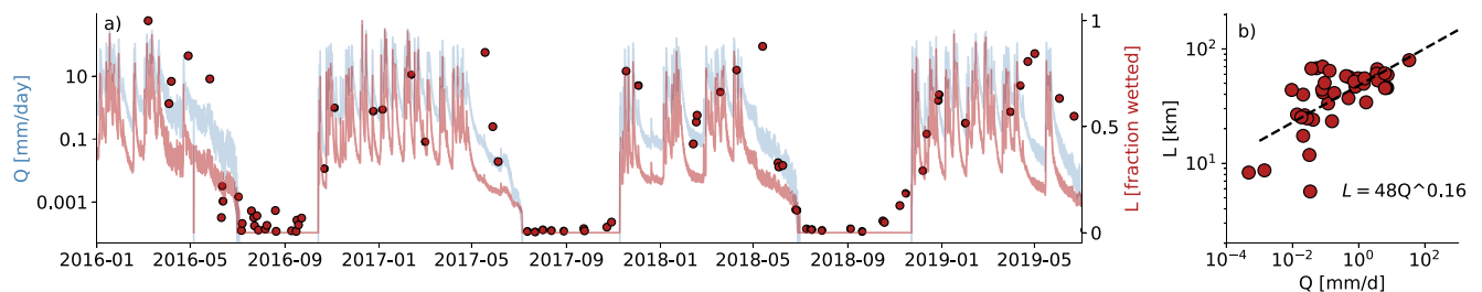
Figure 5. (a) Timeseries of Dry Creek runoff (blue) shown with timeseries of wetted channel length normalized by the maximum predicted length as predicted by a power law fit (red). Red points are discrete values of L calculated from random forest model predictions on RapidEye satellite imagery. (b) The predicted wetted channel extent length as a function of outlet runoff (the power law fit excludes zero flow predictions; R^2 = 0.44 ). The continuous wetted channel prediction (red line in (a)), is estimated from the power law fit in panel (b) using the continuous streamflow timeseries.
