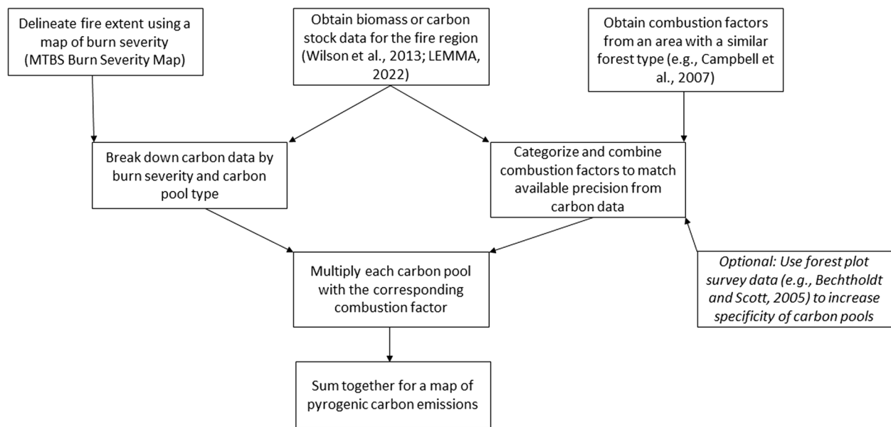
Fig. 2 Conceptual workflow for GIS calculation of total pyrogenic carbon emissions. See supplemental figure 1 for technical workflow including tool names and input and output data
