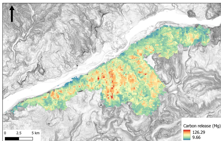
Fig. 4 Total carbon consumed by the Eagle Creek Fire. Red shows areas of high carbon loss and blue shows areas of low carbon loss. Note that areas of high carbon loss correspond to high burn severity as shown in Fig. 1 and/or areas of high pre-burn carbon as shown in Fig. 3
