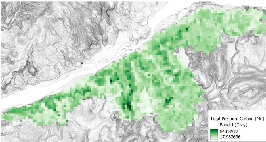
Fig. 3 Total pre-burn carbon stock in the Eagle Creek Fire burn area taken from Wilson et al. (2013)
