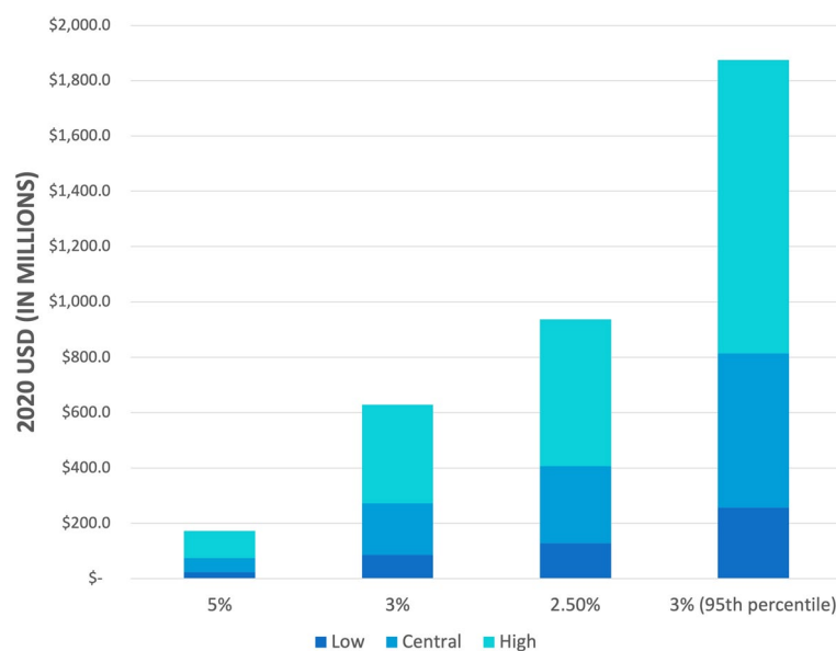
Fig. 6 Economic cost (central scenario, 1.02 Tg) by discount rate, 5%, 3%, 2.5%, and 3% (95th percentile of damages)
