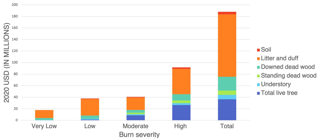
Fig. 5 Economic value of carbon lost by burn severity (x-axis) and vegetation type (color) for the central scenario (1.02 Tg of carbon lost, 3% discount rate). While understory does combust at very low burn severity, the total contribution to carbon loss is small enough that it is not visible on this graph
