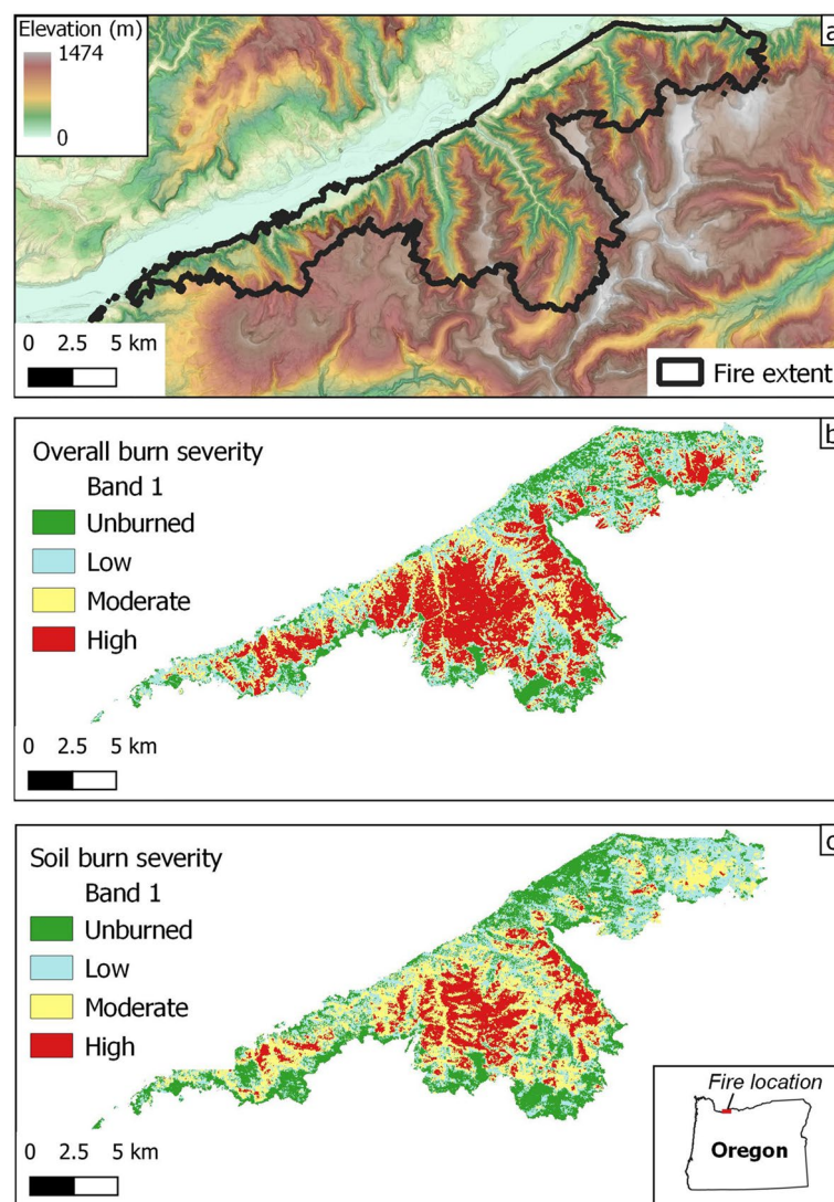
Fig. 1 The Eagle Creek Fire. a Burn perimeter underlain by lidar elevation, b overall burn severity map from Monitoring Trends in Burn Severity (MTBS), and c soil burn severity map from Burned Area Emergency Response (BAER). In b and c , green indicates unburned areas, blue indicates low burn severity, yellow moderate, and red high
