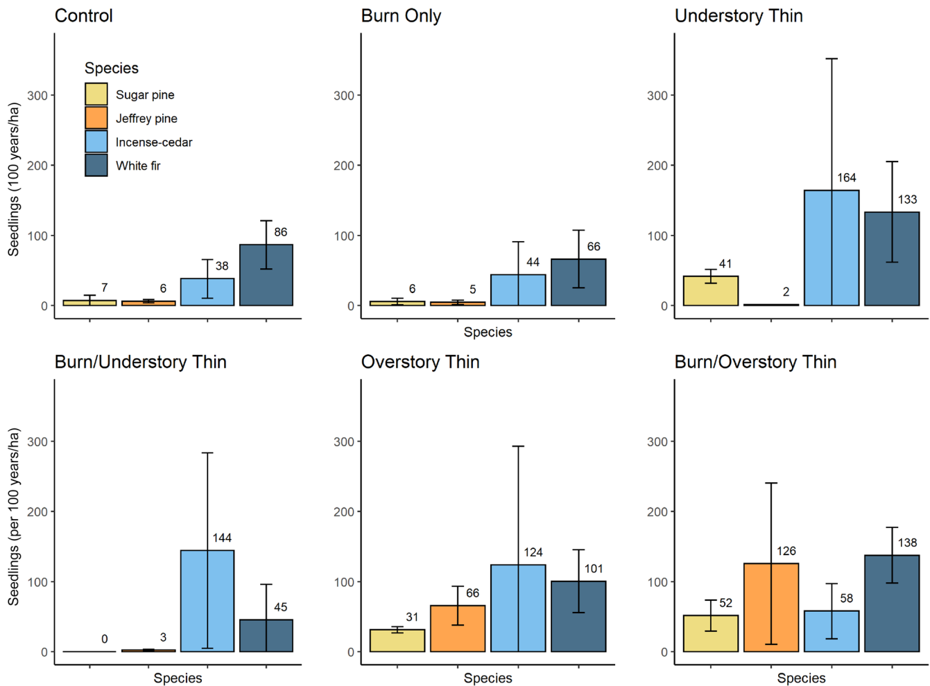
Figure 3. Species-specific rates of midstory recruitment (seedlings surpassing >5 cm DBH) per hectare scaled over 100 years, by treatment. Mean recruitment rates are calculated from records of new trees tagged and mapped plot-wide at each measurement period from 2002–2003 to 2018–2019. Overstory thin and burn/overstory thin plots include recruitment from both planted seedlings and natural seedlings. Error bars represent \pm SDS1.
