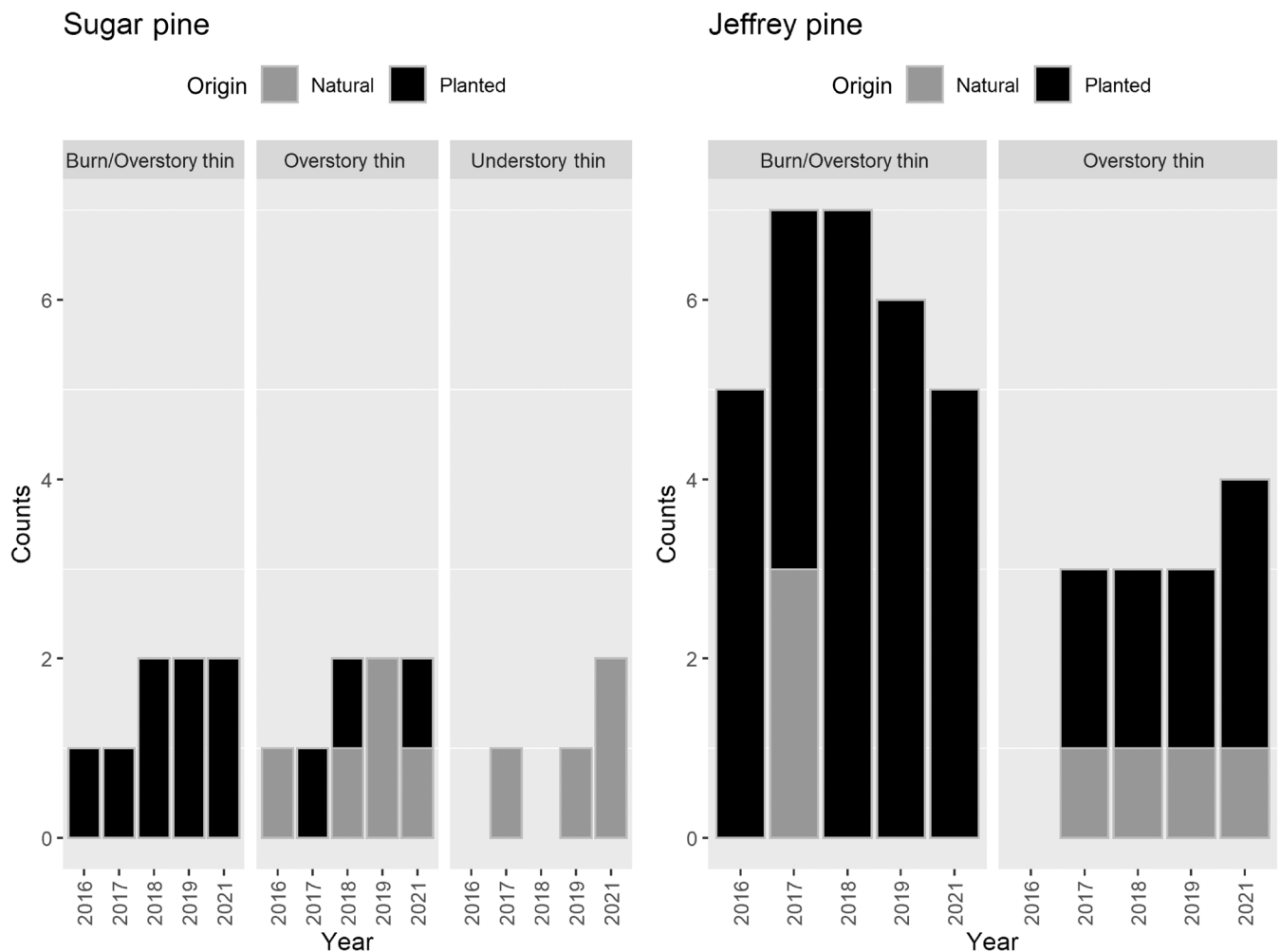
Figure 4. Counts of sugar pine and Jeffrey pine midstory recruitment (>5 cm DBH) detected on regeneration microplots, including only seedlings that crossed this size threshold within the duration of the study (2002–2021). Seedlings were planted in 2002 on overstory thinned plots, with species planted proportionally to pre-treatment overstory dominance. Colors differentiate midstory recruitment counts that were naturally regenerated (gray) from midstory recruitment counts that were originally planted (black). Treatments with no midstory recruitment of these species detected within the duration of the study were not included in the figure.
