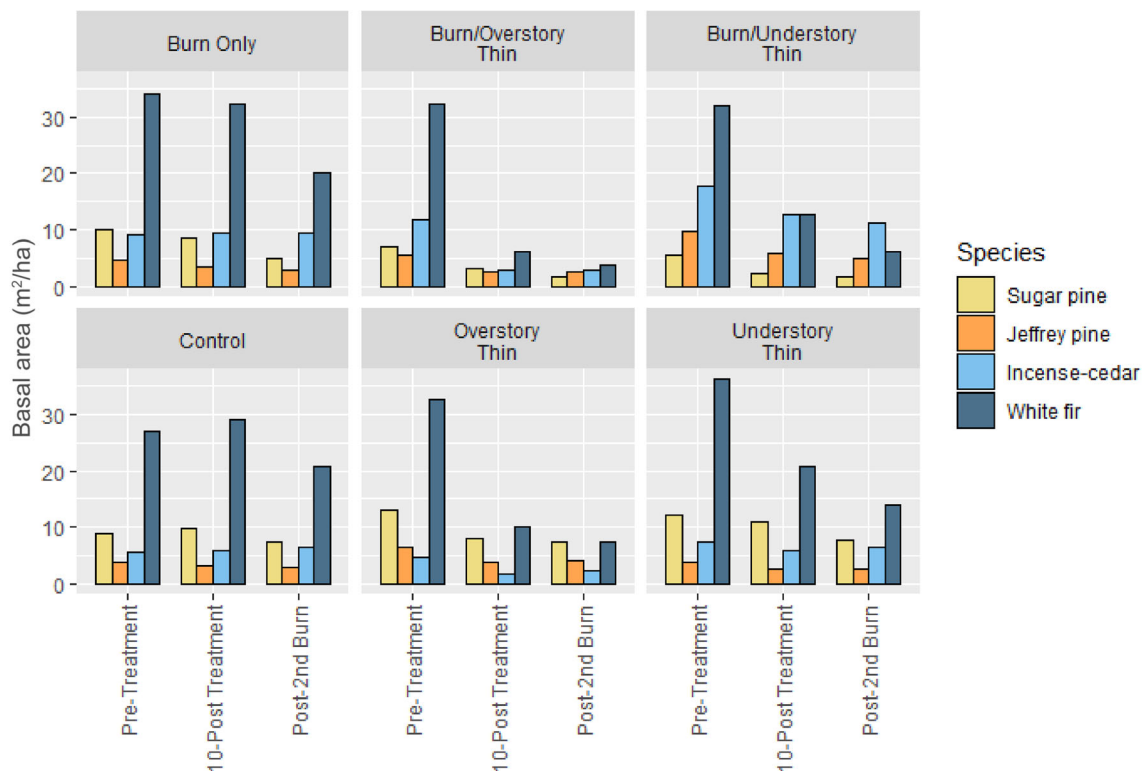
Figure 1. Live overstory basal area by species ( \text{m}^2/\text{ha} ) for each thinning and burning treatment combination, across three sampling periods: pre-treatment (2000–2002), posttreatment/predrought (2011) and postsecond burn/postdrought (2017–2018). Initial thinning and burning treatments occurred in 2000–2001, and a second-entry burn occurred in 2017.
