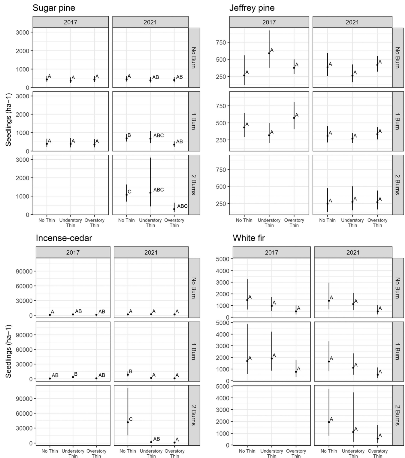
Figure 2. Estimated marginal means seedling density by species for each burn and thinning treatment combination from 2017 (presecond burn) and 2021 (4 years postsecond burn). Marginal means are estimated using a Gamma hurdle, mixed-effects model predicting seedling density, with burn sum, thinning treatment, year, and conspecific basal area as fixed effects. Letters differentiate significant differences ( p < 0.05 ) in pairwise comparisons between treatments and number of burns and are meant to be compared within a year. Error bars represent \pm 95\% CI.
