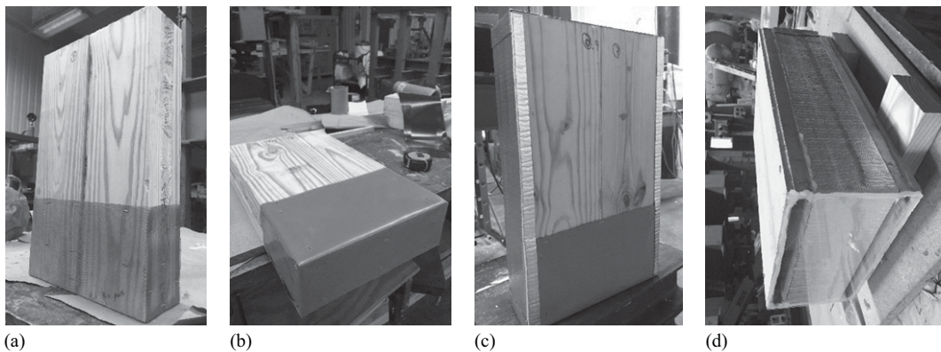
Figure 3. Envelope installation (a) CLT with Termimesh barrier, (b) CLT with Obex11 barrier, (c) CLT edges sealed with aluminum tape, and (d) a complete CLT envelope specimen with spacers and cement board cladding.
