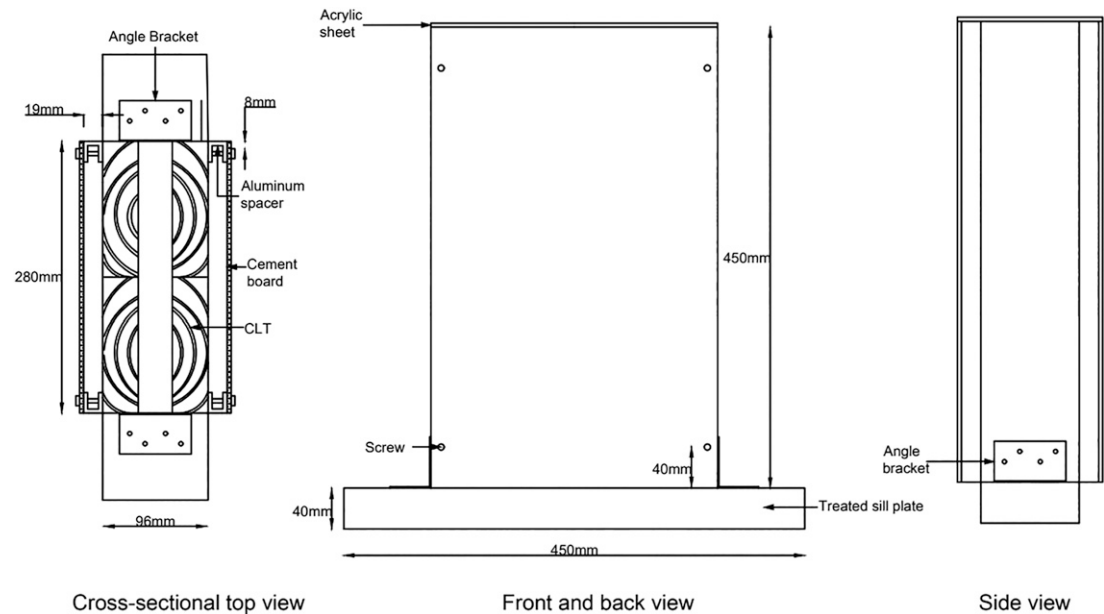
Figure 2. 2D drawing of a CLT envelope specimen.
