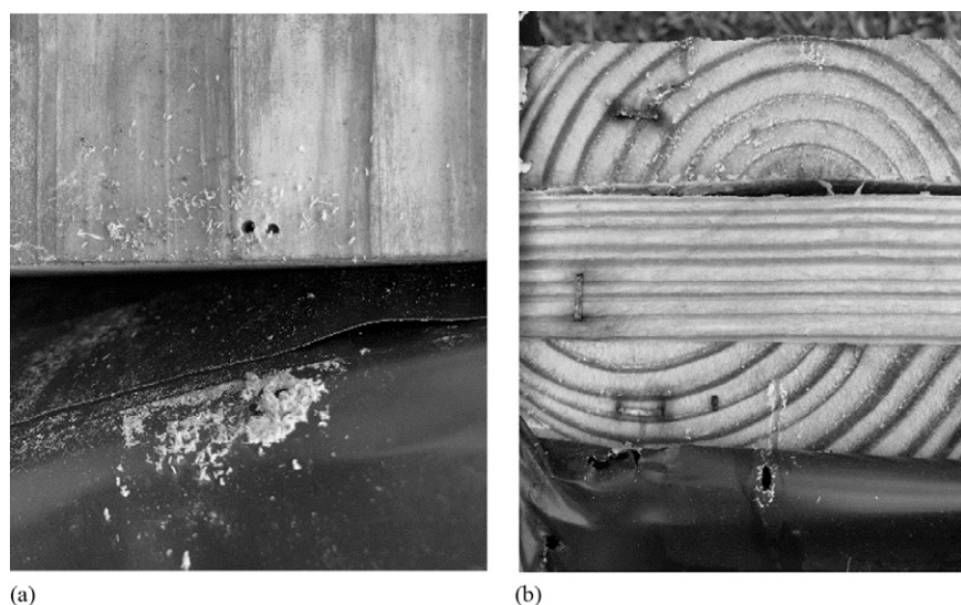
Figure 7. Damage seen in a typical Obex11 specimen showing (a) two beetle puncture holes through the membrane (accumulating sawdust below) and into the face of the CLT near the soil line, and (b) one beetle puncture through the membrane, a bored trail along the CLT base, and laminate separation caused by swelling from trapped moisture.
