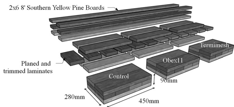
Figure 1. Lumber layout to manufacture one batch of cross laminated timber (CLT) specimens.
