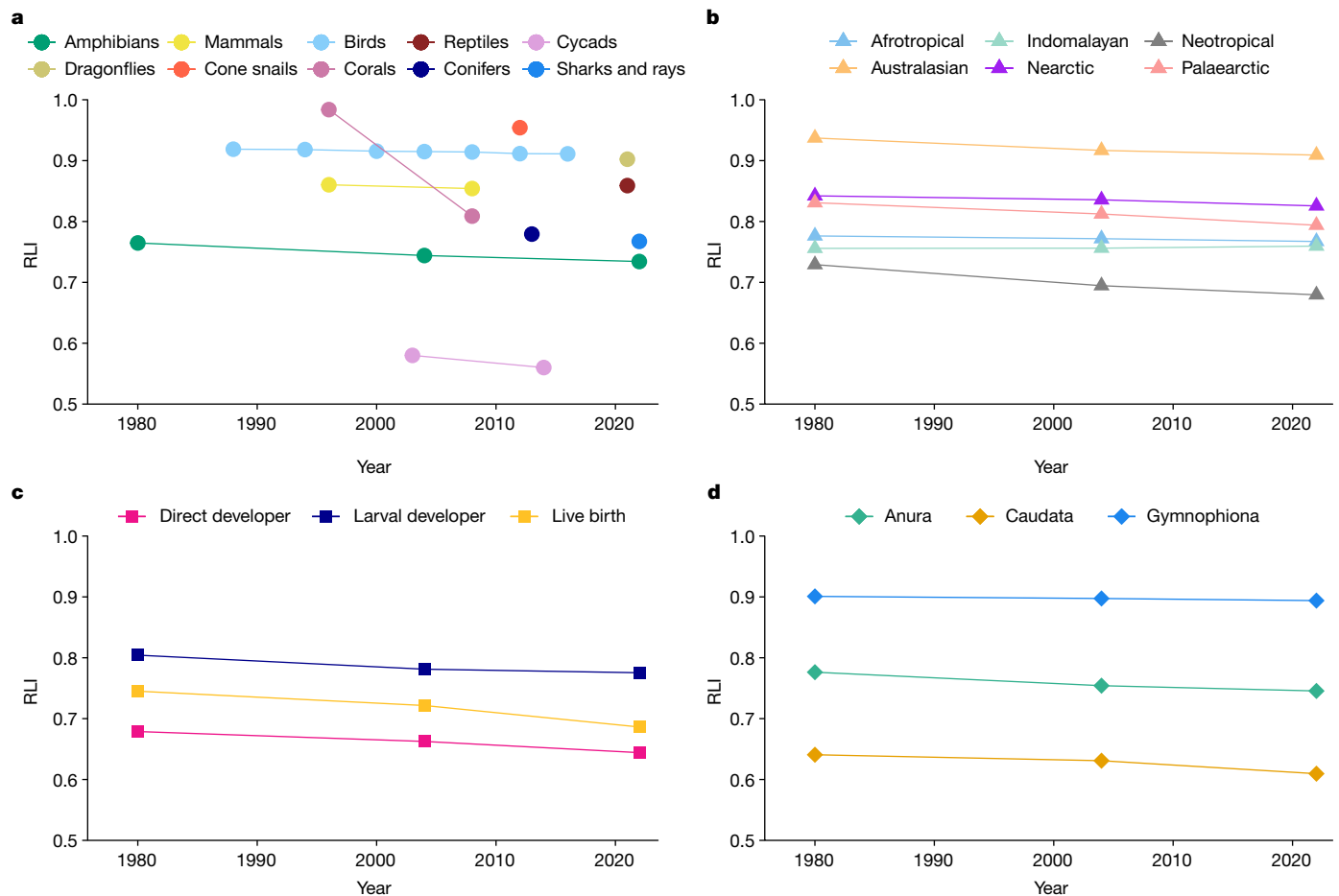
Fig. 3 | RLI is showing trends in overall extinction risk. a , The RLI of all comprehensively assessed taxonomic groups on the IUCN Red List. b , The amphibian RLI disaggregated by biogeographical realm. c , The amphibian RLI disaggregated by breeding strategy. d , The amphibian RLI disaggregated by order.
