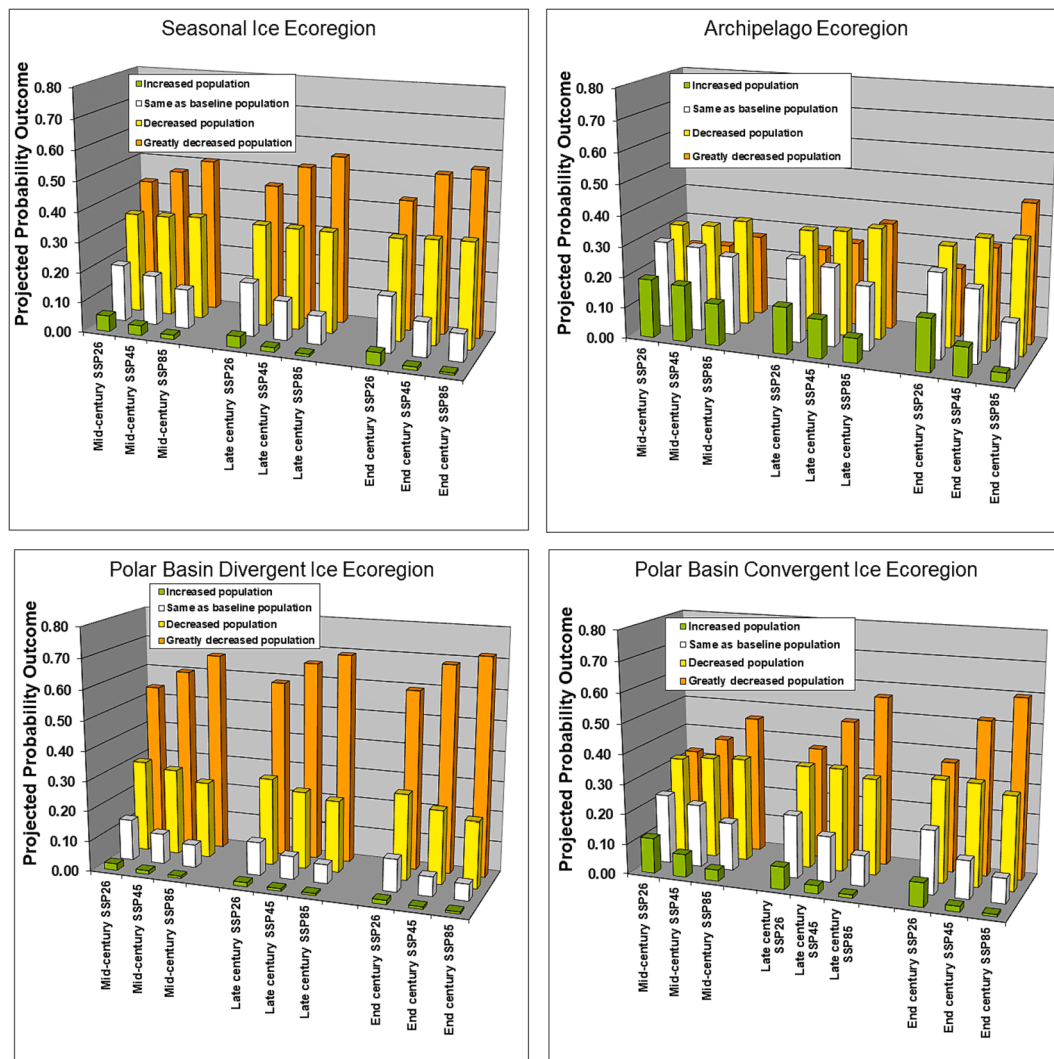
Fig. 1. Projected probabilities of polar bear population outcomes from the Phase III polar bear Bayesian network model (this study) when using CMIP6 (Coupled Model Intercomparison Project Phase 6) sea-ice projections, for four future time periods (see Table 2), under three SSP (Shared Socioeconomic Pathway) greenhouse gas emissions scenarios (2.6, 4.5, 8.5), based on frequency distributions of GCM (global circulation model) outcomes. Greater values denote higher probabilities of four polar bear outcomes (increased, same, decreased, and greatly decreased population) compared to current conditions.
