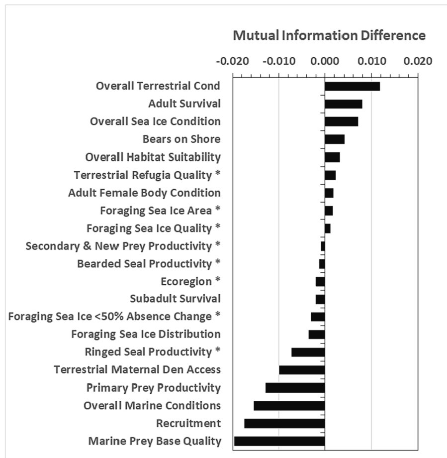
Fig. 3. Changes in sensitivity (mutual information) of variables used in the polar bear Bayesian network models, between the Phase II (Atwood et al. 2016) model using CMIP5 sea ice projections and the Phase III (current study) model using CMIP6 sea ice projections. Greater values denote higher sensitivity in the Phase III model. Shown are variables with > +0.001 or < -0.001 difference in mutual information values. * = input variables.
