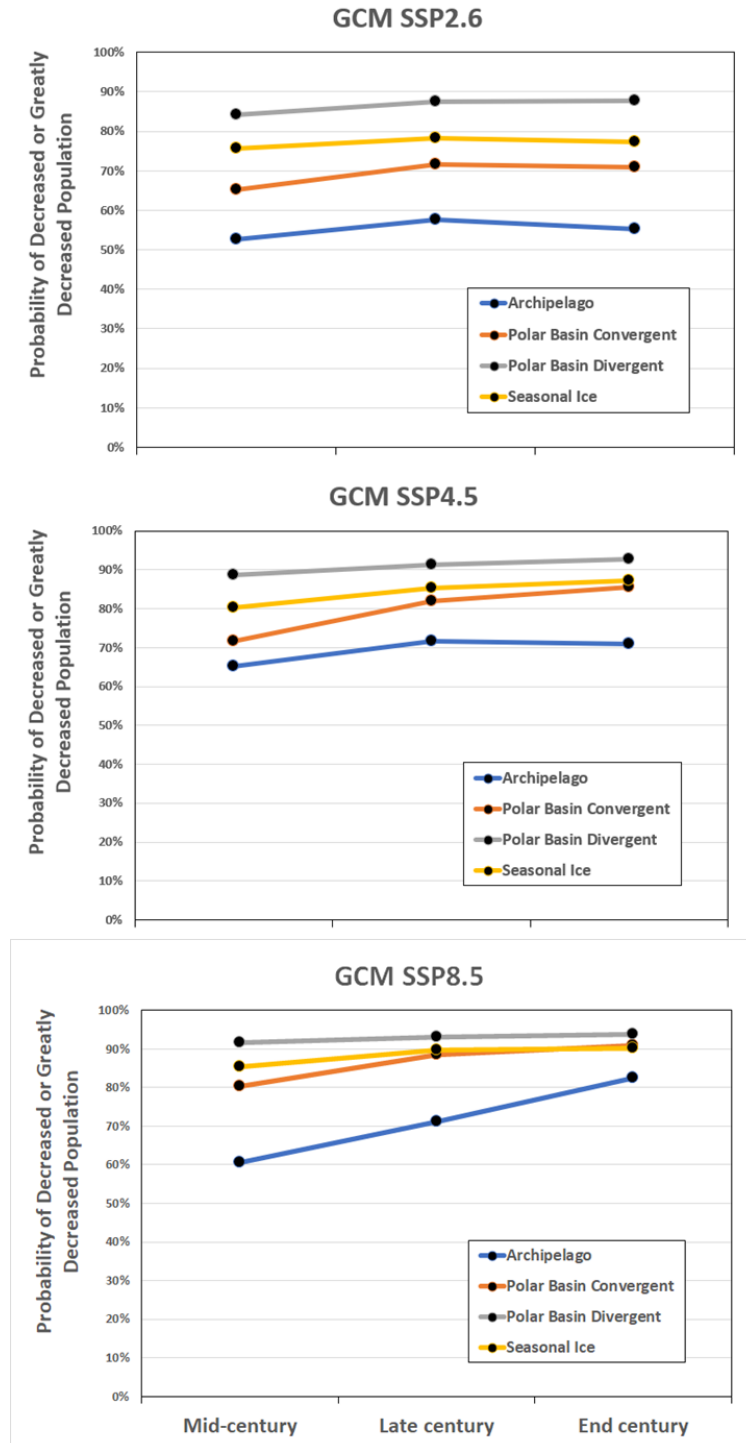
Appendix Figure C2. Summary of projected probabilities of decreased or greatly decreased polar bear populations under the Phase III (current study) Bayesian network model using Coupled Model Intercomparison Project CMIP6 sea-ice projections. Shown here are results by the four ecoregions and three future time periods (see text Table 2), under three SSP (Shared Socioeconomic Pathway) greenhouse gas scenarios (2.6, 4.5, 8.5), based on frequency distributions of GCM (global circulation model) outcomes.
