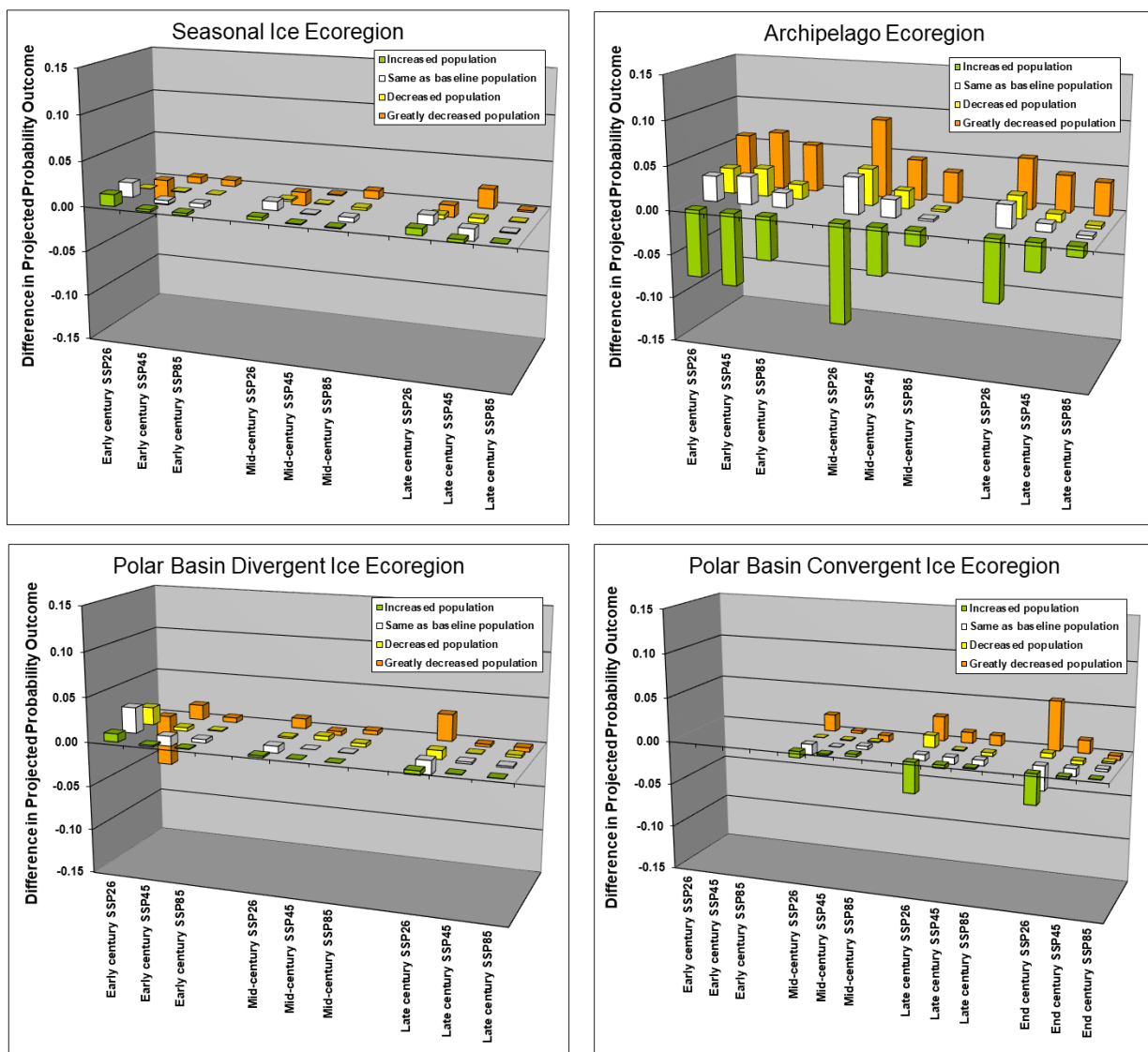
Appendix Figure C3. Differences in projected outcomes of polar bear populations, by ecoregion, time period, and IPCC CMIP (Coupled Model Intercomparison Project) sea-ice projection scenario, using the polar bear Bayesian network Phase II model (Atwood et al. 2016), comparing changes from CMIP5 to CMIP6 sea ice projections from IPCC, for three future time periods. Greater values denote higher probabilities under CMIP6 than CMIP5.
