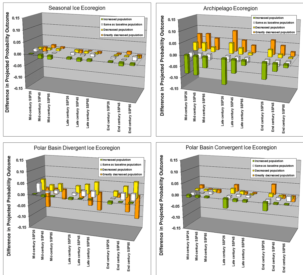
Fig. 2. Differences in projected outcomes of polar bear populations, by ecoregion, time period (see Table 2), and greenhouse gas emissions scenarios, comparing the difference between the Phase III BN model (this study) using CMIP6 sea ice projections and the Phase II BN polar bear model using CMIP5 projections (Atwood et al. 2016), with both model phases using frequency distribution values of the sea-ice projections. Greater values denote higher probabilities of polar bear declines in the Phase III model outcomes than in the Phase II model outcomes. For these comparisons, the CMIP6 emissions scenarios SSP 2.6, 4.5, and 8.5 and the CMIP5 scenarios RCP 2.6, 4.5, and 8.5, were respectively considered analogs.
