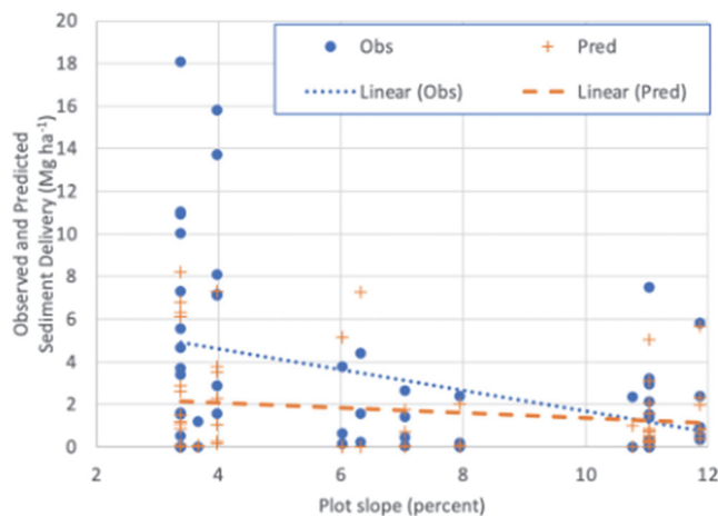
Figure 11. Observed and predicted sediment delivery versus road segment slope for the Fort Benning road erodibility study.
