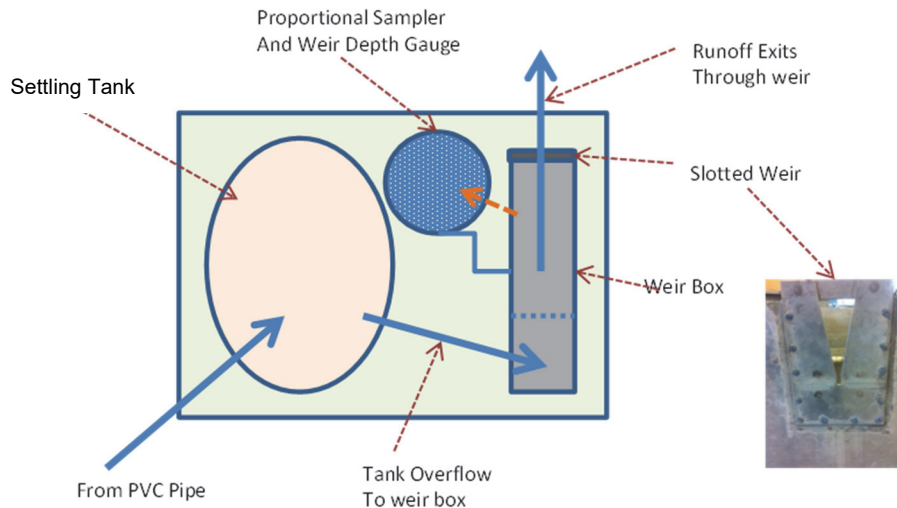
Figure 4. Diagram of components within the sediment box for automatic sampling plots installed at the Fort Benning road erosion study.
