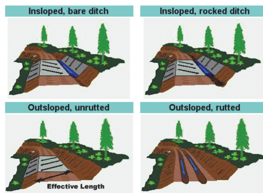
Figure 1. Three road designs for modeling erosion in the WEPP:Road interface plus the insloped design with a vegetated or rock ditch (Elliot, 2004).
