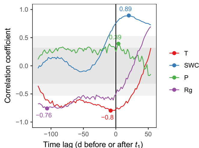
Fig. 4 Spearman's correlation coefficient ( \rho ) between measured final tracheid diameter ( TD_{\max} ; at a weekly resolution, see measured values in Fig. 3a) and environmental variables (T, temperature; SWC, soil water content; P, precipitations; Rg, global solar radiation) averaged following a moving window of 7 d. The lag of the moving window is expressed as the number of d before (negative) or after (positive) the onset of cell enlargement ( t_1 ). Points and corresponding values indicate absolute maximum \rho for each variable. Gray rectangles delimit P -values for which P > 0.001 (light gray) and P > 0.05 (dark gray). When lag = 0 d (vertical solid line), the time window is centered on t_1 . The highest computed positive lag value corresponds to the observed maximum cell enlargement duration (54 d). See scatterplot of the best correlation between TD_{\max} and each environmental variable in Supporting Information Fig. S5.
