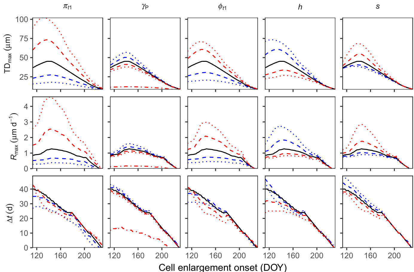
Fig. 6 Predicted enlargement features ( TD_{max} , final tracheid diameter; R_{max} , maximum tracheid enlargement rate and \Delta t , tracheid enlargement duration) of cells formed during the growing season of 2013, using the calibrated model parameters (black) as well as parameters increased (red) or decreased (blue) by 20% (dashed lines) or 40% (dotted lines) relative to their calibrated value ( \pi_{t1} , initial osmotic potential; \gamma_P , yield turgor threshold; \phi_{t1} , initial cell wall extensibility; h , cell wall hardening coefficient; s , cell wall softening coefficient). In the case of \gamma_P , the model was also run using parameter value multiplied by 8 (dash-dot lines) in order to match the average of values reported in the literature (Table 1).
