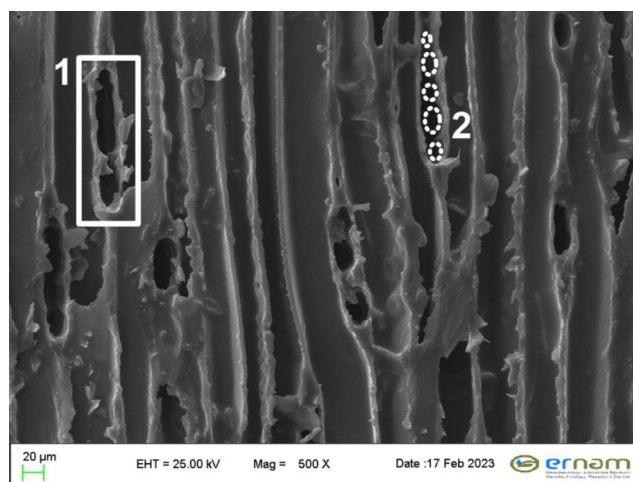
Fig. 7 SEM showing rays remain intact (1), but cell walls are ruptured (2) in charred P. taeda
