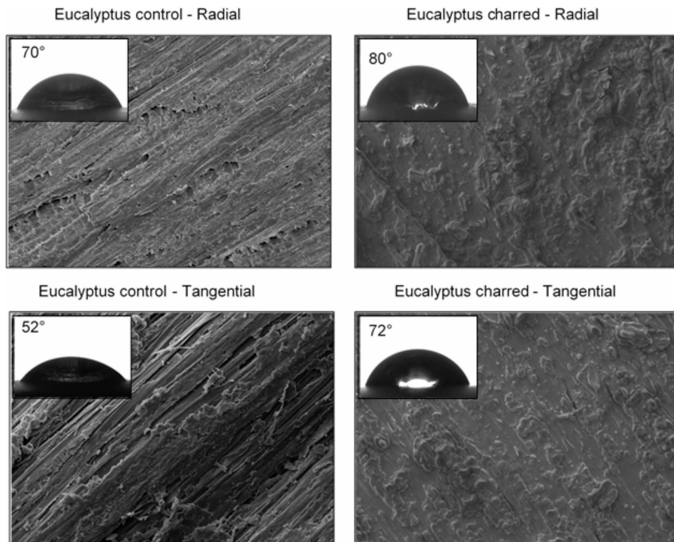
Fig. 4 Contact angle and SEM images of control and charred E. bosistoana specimens on radial and tangential surfaces
