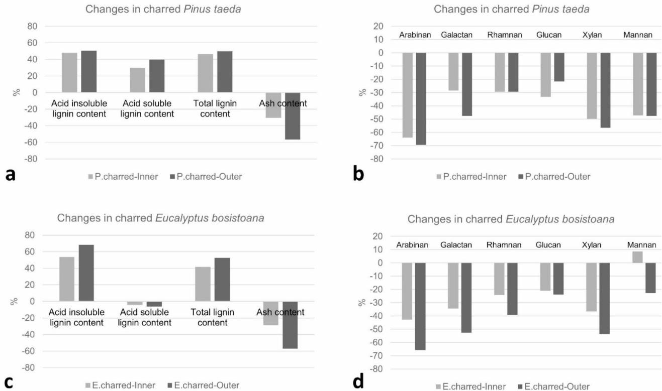
Fig. 1 Percent changes in lignin, ash, and carbohydrate content in charred wood (inner and outer sections) compared to control specimens in a-b) P. taeda and c-d) E. bosistoana
