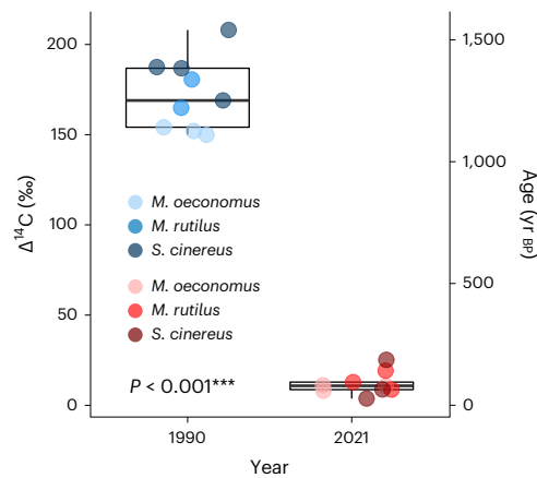
Fig. 3 | Age of carbon assimilated by boreal forest mammals. Radiocarbon values ( \Delta^{14}\text{C} , left) and age (yr BP, right) for small-mammal specimens from 1990 ( N = 9 , blue) and 2021 ( N = 9 , red). Black lines represent median values for each period, boxes represent the interquartile range and whiskers represent minimum and maximum values. Shades represent different species within each period, and P value reflects differences in \Delta^{14}\text{C} between periods determined via two-sided t test.
