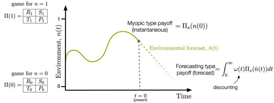
Figure 2. The game payoff matrix \Pi for two alternative strategies depends on the state of the environment, n(t) , which changes over time in response to individuals' actions. A myopic type individual chooses between two alternative strategies based only on the instantaneous payoff of each strategy s in the current environment, \Pi_s(n(0)) . Whereas a more complex type forms a forecast about the future environmental states, \hat{n}(t) using linear extrapolation, and makes decisions that account for expected future payoffs, discounting the future relative to the present. Starting from a population of purely myopic agents, we show that evolution can favor the emergence of forecasting types, even when they pay a cost to produce forecasts.
