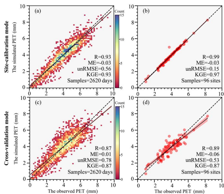
1005 Figure 3: Scatter-plots of observations against simulations aggregated for all of 96 EC sites. (a): Daily comparison in site-calibration mode. (b): Site mean comparison in site-calibration mode. (c): Daily comparison in cross-validation mode. (d): Site mean comparison in cross-validation mode. In these figures, the dash and the solid lines are the 1:1 line and the regression line with the least square method, while the shadow area represents 95% confidence interval.
