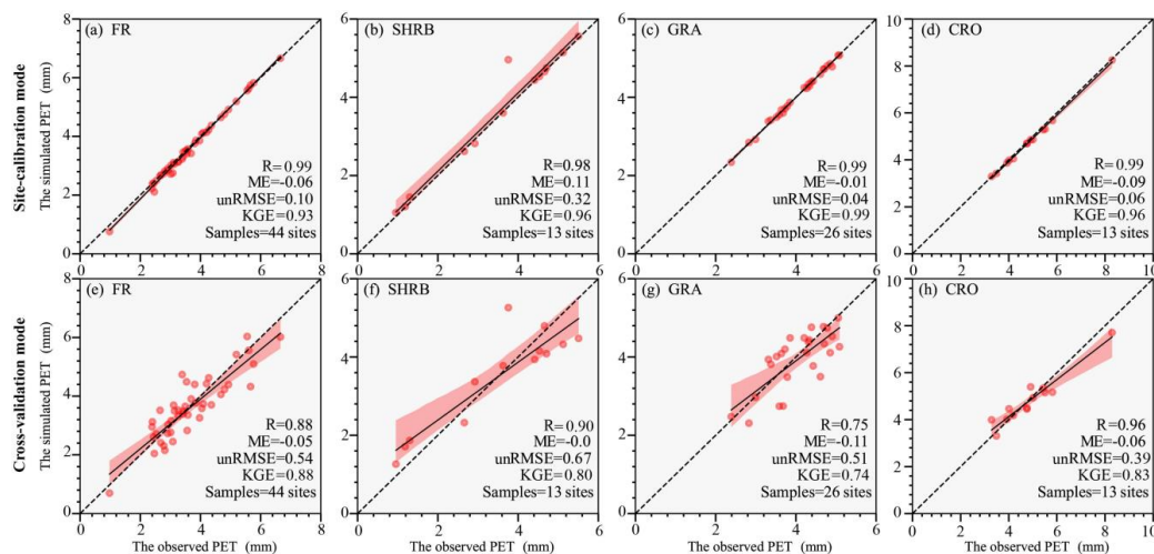
Figure 5: Scatter-plots site mean observations against simulations for each LULC type. (a–d): Comparison in site-calibration mode. (e–h): Comparison in cross-validation mode. In these figures, the dash and the solid lines are the 1:1 line and the regression line with the least square method, while the shadow area represents 95% confidence interval.
