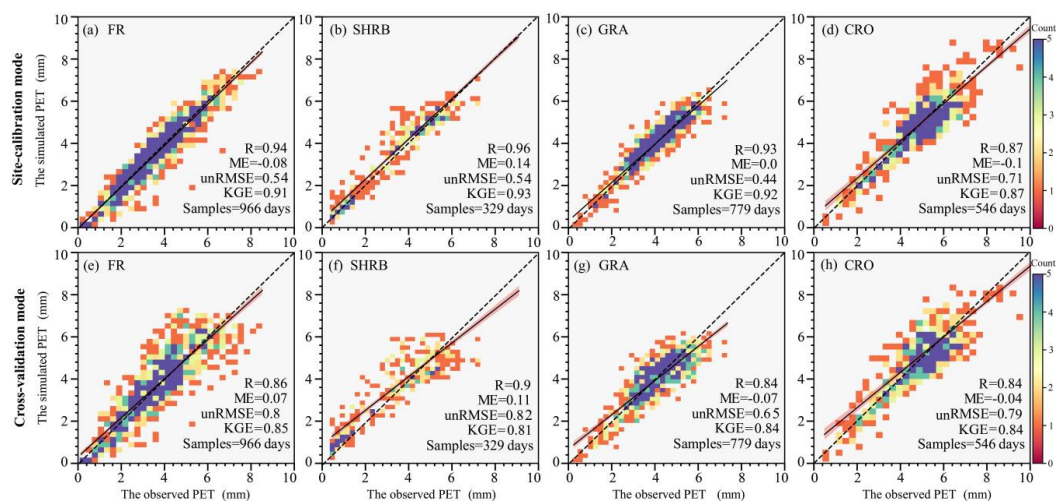
Figure 4: Scatter-plots of daily observations against simulations aggregated for different LULC types. (a–d): Comparison in site-calibration mode. (e–h): Comparison in cross-validation mode. In these figures, the dash and the solid lines are the 1:1 line and the regression line with the least square method, while the shadow area represents 95% confidence interval.
