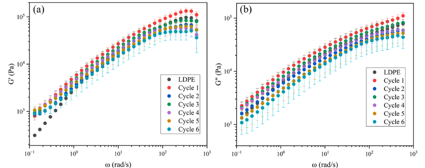
Fig. 12. Storage modulus (a) and loss modulus (b) vs frequency plots of LDPE and the reprocessed blend.
