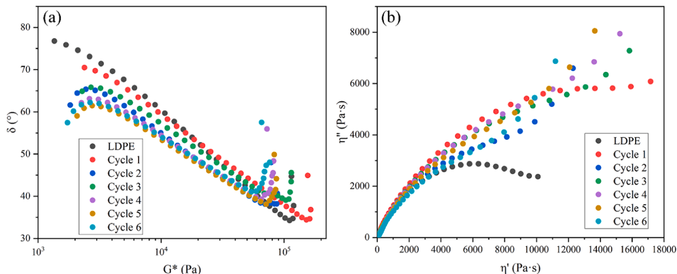
Fig. 14. Van Gorp Palmen (vGP) plots (a) and Cole-Cole plots (b) of LDPE and the reprocessed blend.
