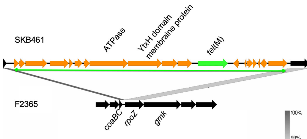
FIG 1 Genomic organization of the Tn916.1039-harboring region in the bear-derived Listeria monocytogenes strain SKB461. The Tn916-like element Tn916.1039 is indicated with the green double-pointed arrow. Open reading frames (ORFs) conserved in the reference strain L. monocytogenes F2365 are in black. The tetracycline resistance determinant tet(M) is in green. The gray scale indicates nucleotide sequence identity (%) in the flanking sequences. Comparative genomic organization was determined as described in Materials and Methods and visualized using EasyFig.
