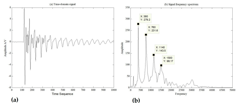
Figure 18. Typical acoustic signal of a wood member obtained in resonance-based acoustic measurement (a) and the corresponding frequency spectrum obtained through FFT analysis (b).
