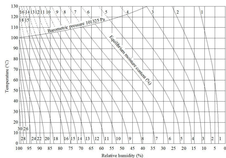
Figure 23. Hygroscopic isotherms for Sitka spruce at different temperatures based on Kollmann and Côte [153]. Redrawn by the Timber Construction Research Group-UPM.
