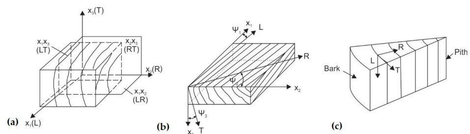
Figure 5. Main directions for wood. (a) Main axes; (b) Polar coordinates for the influence of the grain angle (LR, LT) and the annual ring position, ring angle (RT); (c) Pure orthotropic system (main direction L —longitudinal, R —radial, T —tangential). Source [15], (courtesy of Carl Hanser Verlag GmbH & Co. KG).
