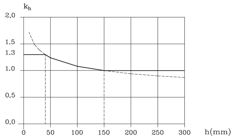
Figure 27. Depth factor k_h , in sawn timber. Design value in a continuous line and Equation (4) in a dotted line (from Arriaga et al. [179]).
