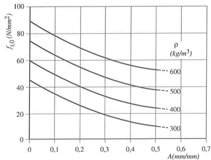
Figure 11. Effect of knot ratio and density on tensile strength [63], courtesy of P. Glos.
