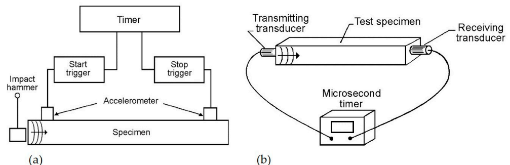
Figure 17. TOF acoustic measurement system used to measure longitudinal wave velocity in a wood member through (a) mechanical impact, and (b) ultrasonic waves (source: [87], courtesy of the USDA Forest Service, Forest Product Laboratory, Madison, WI, USA).
