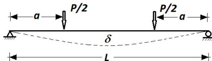
Figure 14. Standard bending test for full-size sawn timber with two-point loading.
