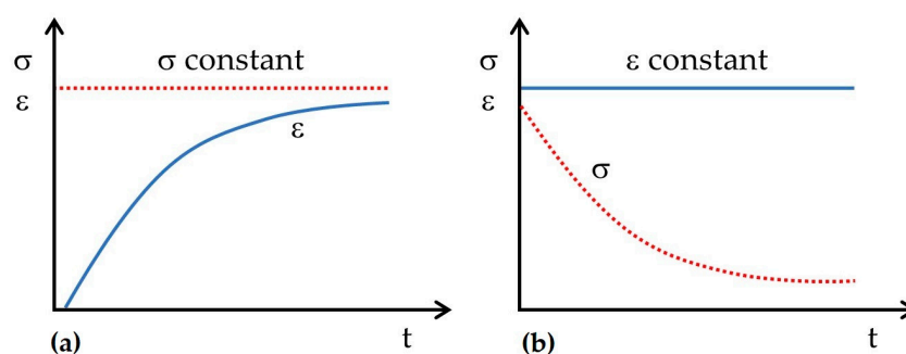
Figure 21. Rheological behaviour and creep effect of wood and wood-based materials under static load. (a) Constant stress and unitary deformation including creep factor. (b) Relaxation of stress under constant unitary deformation (based on [15]).
