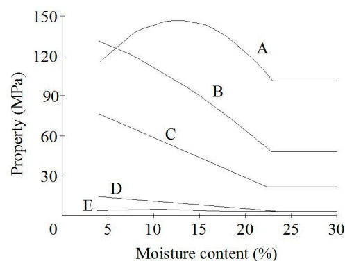
Figure 24. Effect of moisture content on wood strength properties based on the Wood Handbook [60]. A—Tension parallel to the grain, B—Bending, C—Compression parallel to the grain, D—Compression perpendicular to the grain, and E—Tension perpendicular to the grain. Redrawn by the Timber Construction Research Group-UPM.
