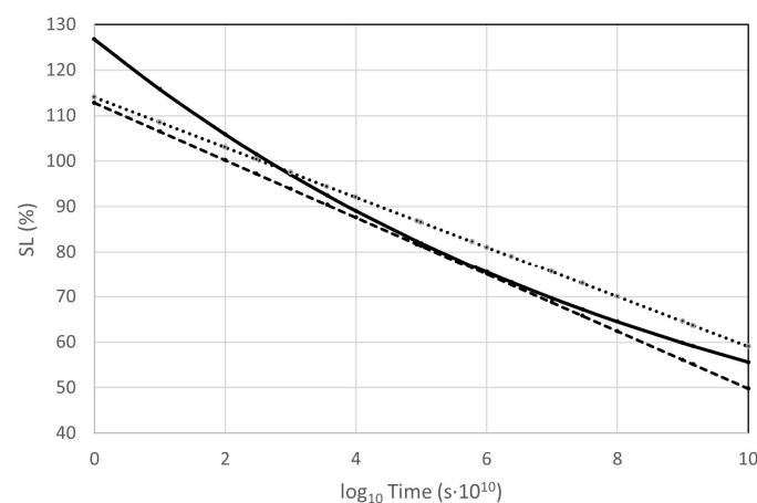
Figure 22. Relation of the duration of the load to the stress level. Madison curve (solid line), Wood curve (dashed line), and Madsen curve (dotted line) [140].
