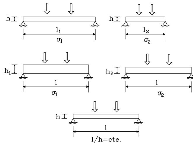
Figure 26. Length and depth effect in bent members (from Arriaga et al. [179], based on Madsen and Nielsen [50]).
