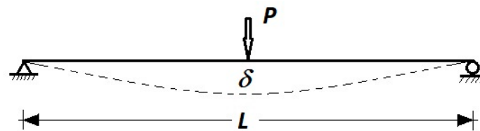
Figure 13. Standard bending test for small clear wood with centre-point loading.
