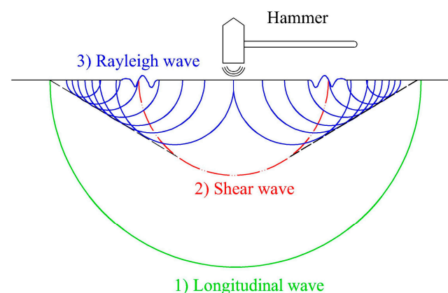
Figure 15. Types of stress waves in semi-infinite elastic material (based on [96]).
