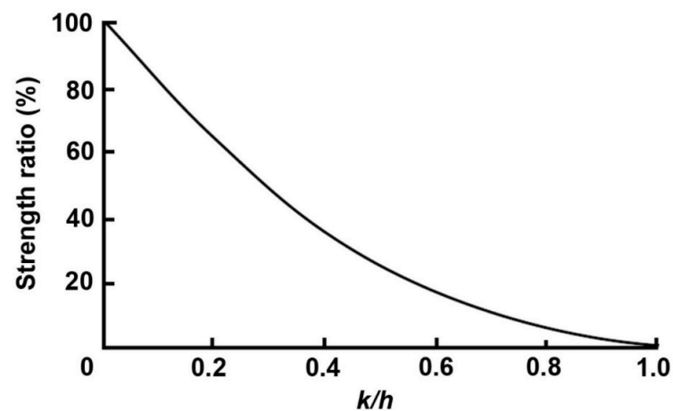
Figure 12. Relation between bending strength ratio and size of edge knot (k) expressed as a fraction of face width (h) (source: [60] courtesy of the USDA Forest Service, Forest Product Laboratory, Madison, WI, USA).
