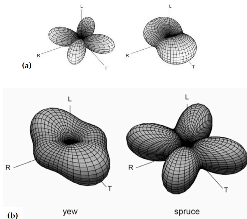
Figure 7. Deformation body of wood. (a) Spruce and beech wood in normal climate according to ([33], source [15], (courtesy of Carl Hanser Verlag GmbH & Co. KG, Munich); (b) Yew and spruce under tensile load [17] (Courtesy of D. Keunecke).
