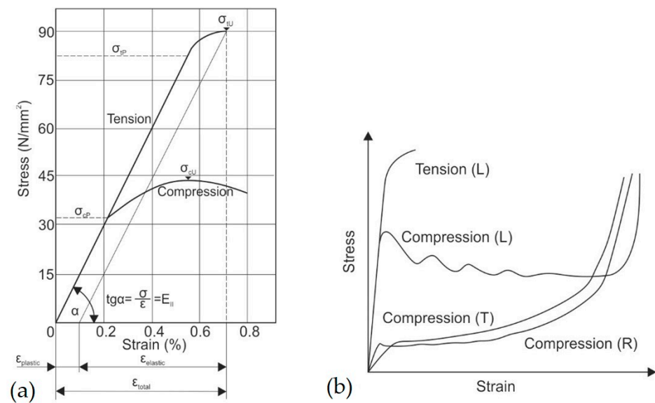
Figure 4. Stress-strain diagram of solid wood [15] (courtesy of Carl Hanser Verlag GmbH & Co. KG, Munich): (a) Solid wood under tensile and compressive stress in the direction of the fibre. (b) Tension and compression parallel and perpendicular to the fibre direction according to [22].
