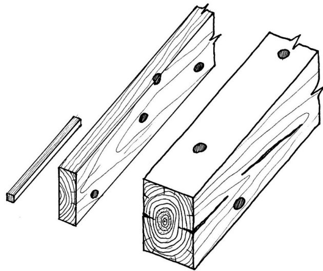
Figure 9. Left to right: Small-size clear specimen, Structural-size medium and large cross-section (Credit: GICM-UPM).
