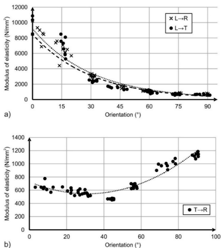
Figure 6. Influence (a) of the fibre load angle (LR, LT) and (b) of the annual ring inclination (RT) on the modulus of elasticity of ash wood according to Clauß et al. modified [34].
