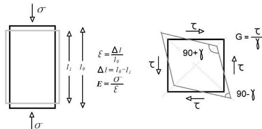
Figure 3. Elongation of a bar under compression stress and angle distortion caused by shear stresses.
