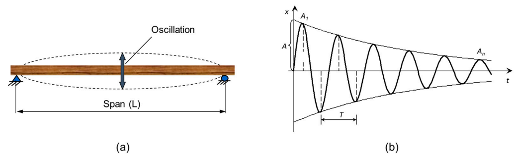
Figure 20. Transverse vibration of a simply supported wood member (a) and the waveform of free vibration (b).
