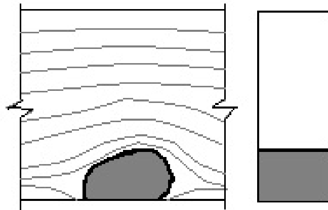
Figure 10. Cross-sectional reduction due to edge knots.
