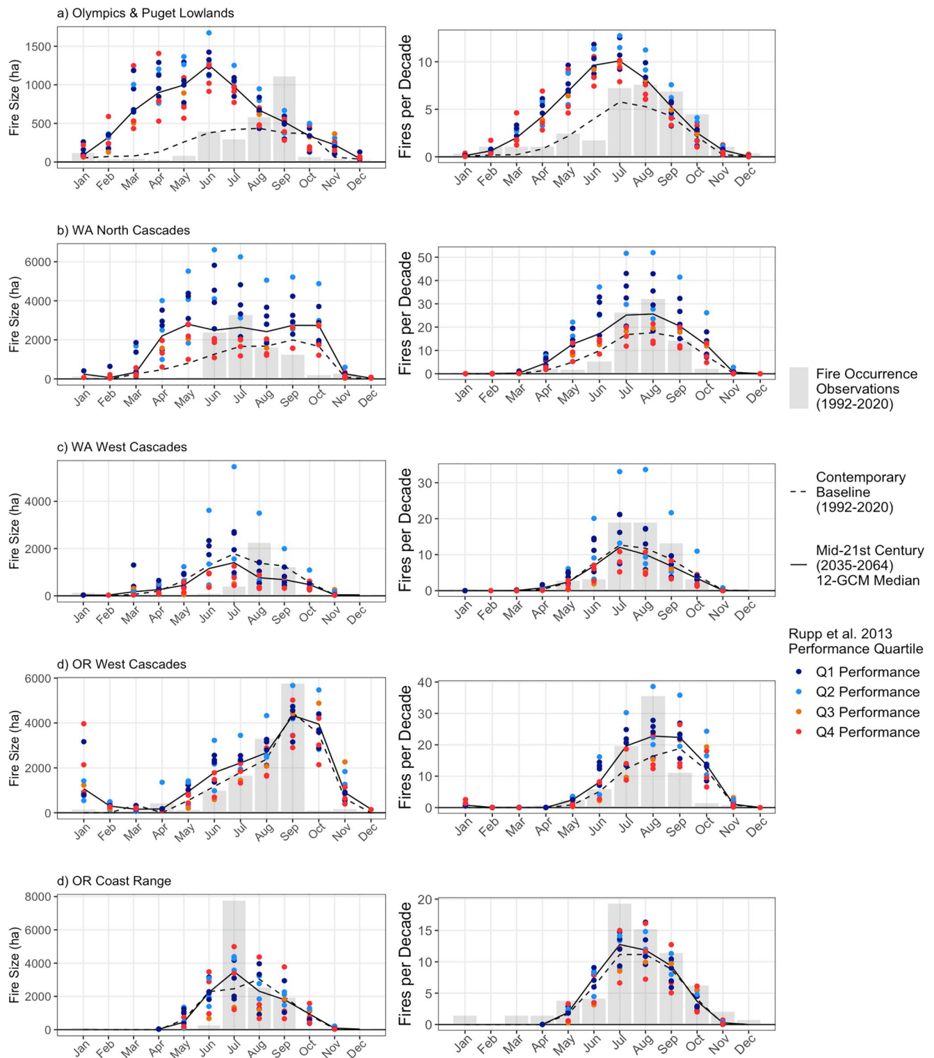
Figure 7. Monthly distribution of simulated fire size and number of fires per decade for the contemporary baseline (1992–2020) and mid-century future (2035–2064) scenarios. For mid-century scenarios, the median monthly value of the 12 GCM-based simulations is drawn as a solid line, and individual points for each simulation are color-coded by their Rupp et al., 2013 GCM performance ranking quartile as in Figures 3, 5 and 6. Observations from the historical fire occurrence database are shown as gray bars in background.
