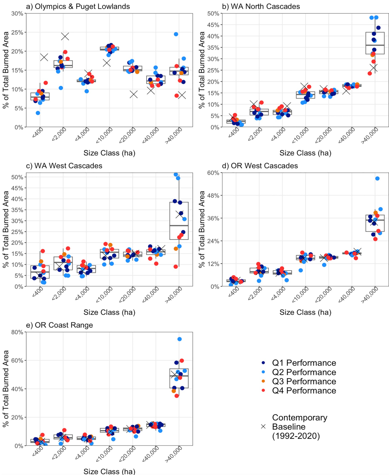
Figure 6. The proportion of total area burned by each of 7 size classes. Boxes mark the median and first/third quartiles; whiskers extend to \pm 1.5 \times IQR. Each point is an individual GCM-based simulation, colored by Rupp et al. (2013) GCM performance ranking quartile as in Figures 3 and 5. In the appendix, see companion Figure S7 in Supporting Information S1 which instead plots the proportion of the fire occurrence area (FOA) burned by size class per decade.
