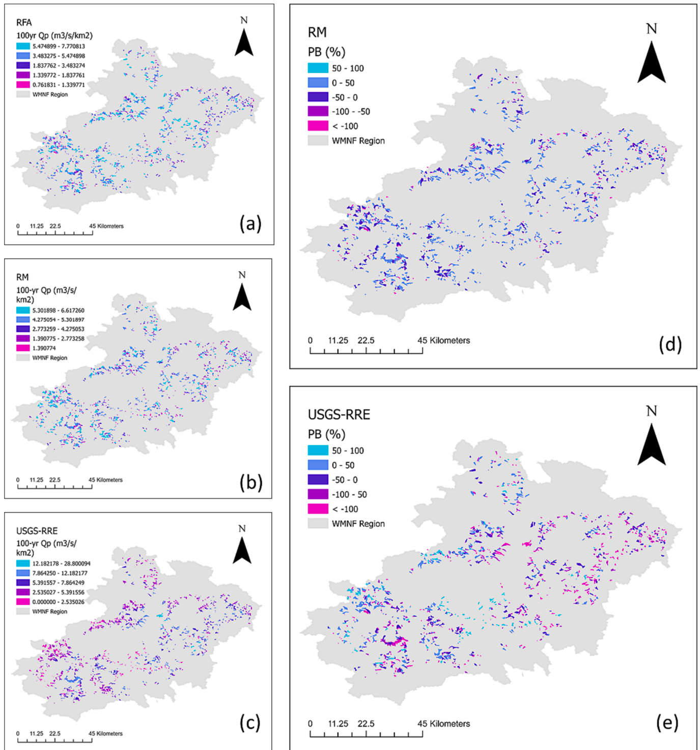
Fig. 6. Spatial map showing the (a–c) 100-yr Q_p (in m^3/s/km^2 ) estimated by the (a) RFA, (b) RM, and (c) USGS-RRE methodology, and (d–e) the PB (in %) for the 100-yr Q_p estimated by (d) RM and (e) USGS-RRE methodology compared to RFA for the HUC16-20 (gauged and ungauged) watersheds within the WMNF that intersects with the culverts and RSCS.
