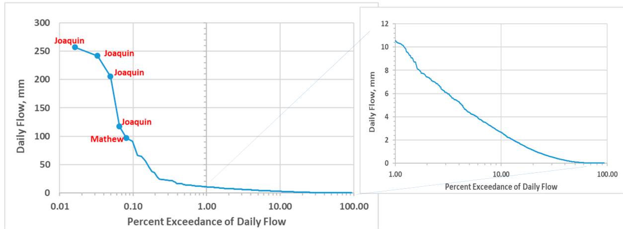
Figure 6. Daily flow frequency duration curves. A closer view of the lower exceedance values is shown at right.
