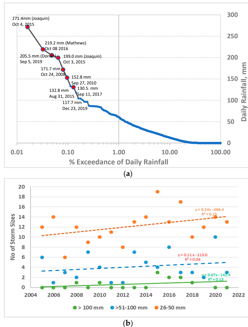
Figure 5. (a) Daily rainfall frequency–duration curves and (b) annual trends in the number of storm sizes for three different categories of rainfall: rainfall storm totals > 100 mm, storm totals between 51–100 mm, and storm totals between 26–50 mm.
