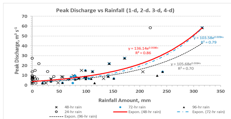
Figure 8. Relationship of peak discharge with rainfall amounts for 24, 48, 72-, and 96 h durations observed during the 2005–2021 period without the estimated discharge of extreme event on 5 October 2015.
