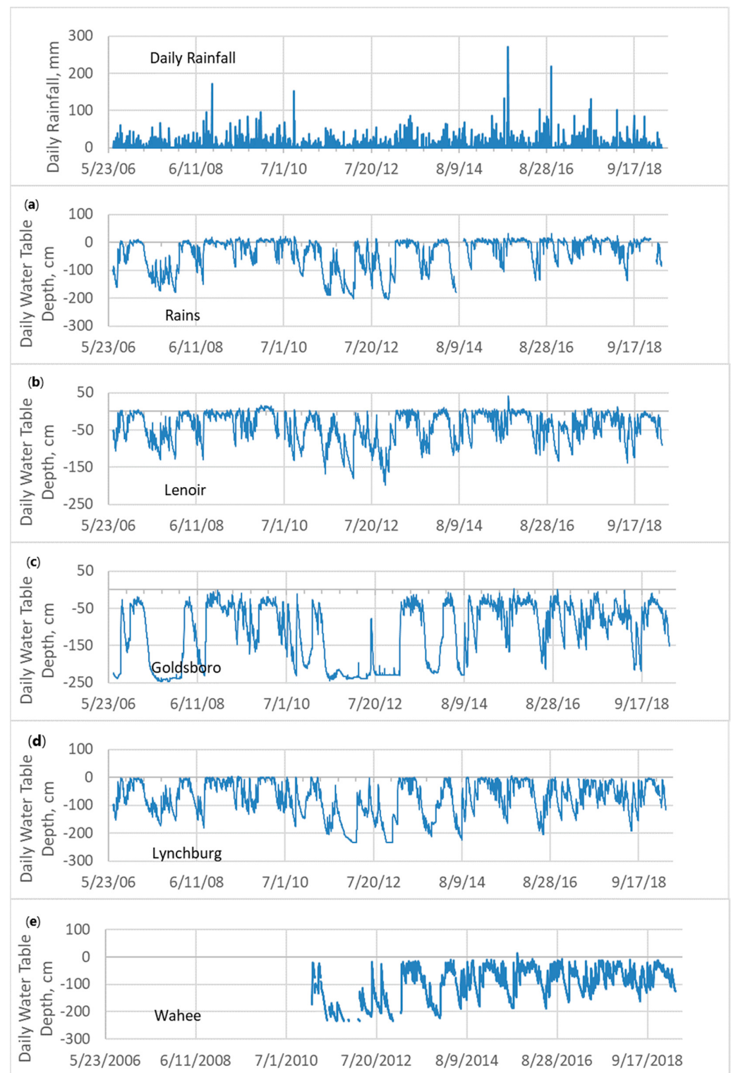
Figure 9. Daily water table from 9m shallow groundwater wells on five dominant soil types: (a) Rains, (b) Lenoir, (c) Goldsboro, (d) Lynchburg, and (e) Wahee for 2006 to 2021 period.
