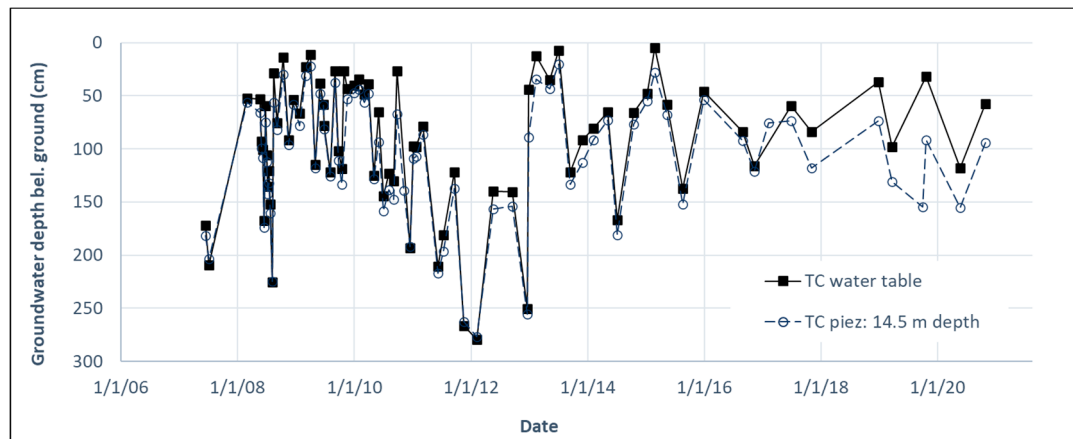
Figure 10. Groundwater head data (2006–2020) for the upper Turkey Creek location. Water table and piezometric head for a 14.5-m deep piezometer are shown. Lenoir soil series (clayey Aeric Paleaquults). The vertical separation of the two data series indicates a consistent albeit small downward hydraulic gradient between the water table and deeper groundwater system.
