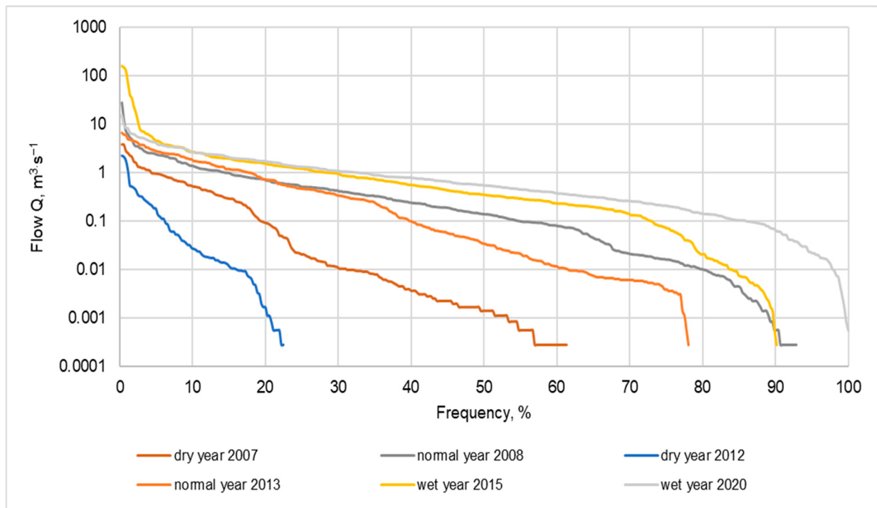
Figure 7. Daily flow rates frequency duration curves for dry years of 2007 and 2012, normal years of 2008 and 2013, and wet years of 2015 and 2020.
