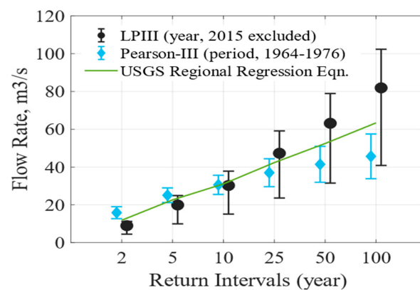
Figure 12. Comparison of 2, 5-, 10-, 25-, 50-, and 100-year design flow rates estimated using on-site annual maximum peak flow rate with LPIII distribution fit, results from Pearson Type III (published in Amatya and Radecki-Pawlik (2007) [95]), and regional USGS regression equation. The error bars indicate 5–95% confidence intervals for the LPIII distribution fit.
