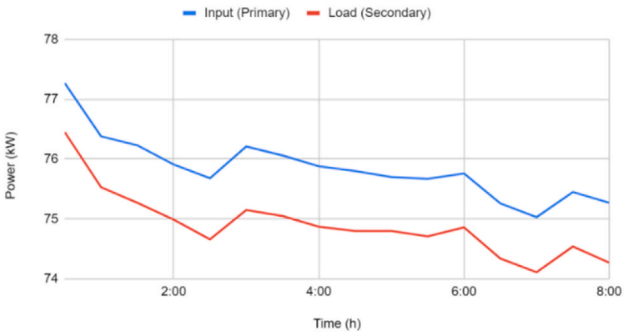
Fig. A5. Power at primary and secondary side of transformer during loading..
