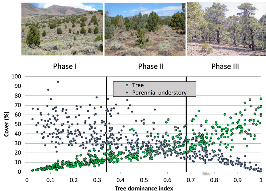
Fig. 6 The change in tree dominance across the phases of pinyon and juniper expansion. In phase I, trees are present but shrubs and herbs are the dominant vegetation influencing ecological processes; in phase II, trees are codominant with shrubs and herbs and all three vegetation layers influence ecological processes; in phase III, trees are the dominant vegetation on the site and are the primary influence on ecological processes (Miller et al. 2005). The tree dominance index (TDI) is used as a quantitative measure of the relative dominance of pinyon and juniper based on the proportion of tree canopy cover to the summation of shrub and perennial grass (or herb) cover and is calculated as: tree cover / [tree + shrub + tall perennial grass cover]. Figure from Miller et al. (2019)
