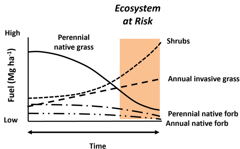
Fig. 4 A conceptual model of the changes in fuel types over time in sagebrush-dominated ecosystems that are not experiencing pinyon-juniper expansion. Increases in shrub fuels over time occur due to a combination of succession, fire suppression, or livestock grazing and may result in decreases in perennial native grasses, perennial native forbs, and annual native forbs. In warmer and drier ecosystems with relatively low resilience and resistance, perennial native grasses and forbs decrease while invasive annual grasses increase. Ecosystems with high levels of shrub and/or invasive annual grass fuels are at risk of transitioning to alternative states dominated by the invaders after wildfires or management treatments that remove shrubs as indicated by the shaded area
