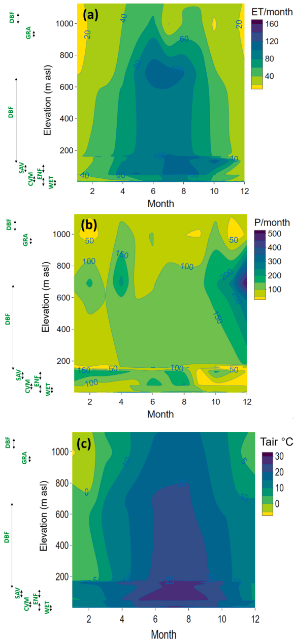
Fig. 7. Contour plots of the seasonal variation in (a) ecosystem evapotranspiration (ET, mm), (b) precipitation (P, mm) and air temperature ( T_{air} , °C) as a function of elevation (m, asl) across different ecosystem types in the U.S. Southeast including GRA (Grasslands), DBF (Deciduous Broadleaf Forests), CVM (Cropland Vegetation Mosaics), ENF (Evergreen Needleleaf Forests), WET (Wetlands), and SAV (Savannas).
