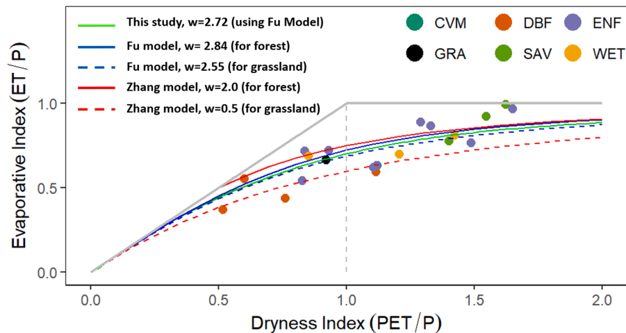
Fig. 9. The Budyko curves derived using the mean annual data of ET, PET, and P across the flux sites in the U.S. Southeast. The thick gray and dashed gray lines show the physical boundaries of the curve where the dryness index (PET/P) increases with the evaporative index (ET/P) over the energy-limited region and where ET/P is independent of PET/P over the water-limited region. Comparison of the Budyko curves derived using the Fu et al., 1981 (blue line), Zhang et al., 2001 (red line), and the model developed in this study by optimizing the w (plant-available water coefficient) to 2.67 (green line). Ecosystem type is denoted by colored circles in each panel as GRA (Grasslands), DBF (Deciduous Broadleaf Forests), CVM (Cropland Vegetation Mosaics), ENF (Evergreen Needleleaf Forests), WET (Wetlands), and SAV (Savannas).
