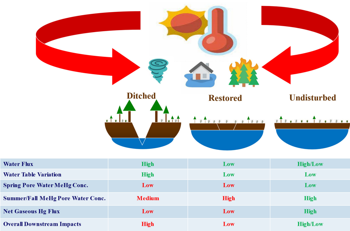
Figure 1. Mercury cycling interactions with climate and ditched, restored, and undisturbed peatlands. Climate interactions include warming and those impacts of extreme events such as storms (tornadoes and hurricanes), flooding, and fires resulting from droughts. The associated table indicates the direction of pore water MeHg concentrations, and our relative confidence is denoted by color with green denoting confident and red denoting little confidence because the interaction is untested. The water flux and overall downstream impact from undisturbed peatlands are high when directly connected to surface waters (e.g., streams) and low for seepage wetlands with no outlets. Although the images are small, the ditched and undisturbed peatlands include sedges while the restored peatland does not.
