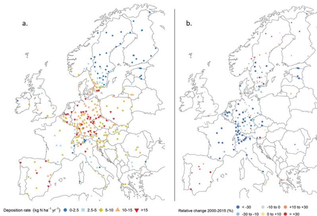
FIG. 2.2 Map of ICP forests intensive monitoring sites showing (a) mean throughfall deposition of inorganic N for the period 2011–15 and (b) relative change in throughfall inorganic N deposition during the period 2000–15. This figure is reused from Schmitz et al. (2018) with permission.
