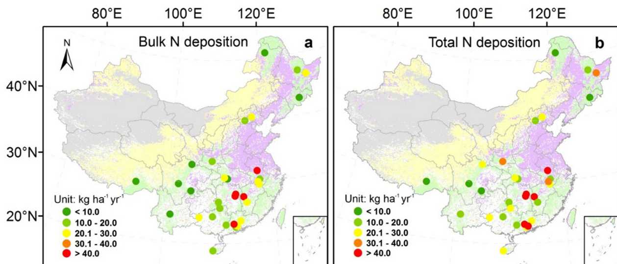
FIG. 2.6 Spatial patterns of (a) bulk N deposition and (b) total N deposition (as a sum of N fluxes in throughfall and stemflow) in China's forests. The background shading in light green, yellow, purple and gray indicate the distribution of forest, grassland, cropland and other land covers, respectively. Reproduced from Du, et al. (2016) under the Creative Commons Attribution 3.0 License.
