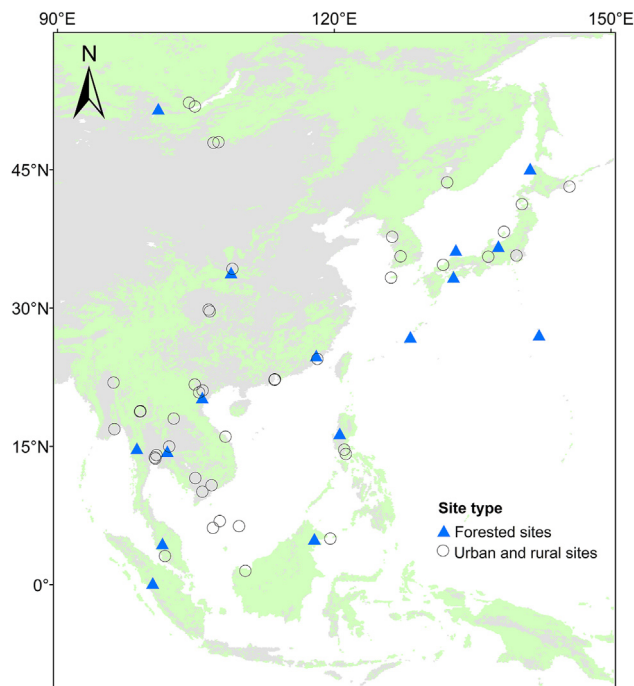
FIG. 2.5 Spatial distribution of EANET sites ( http://www.eanet.asia ) in forested and non-forested environments. The green and gray shading areas indicate the distributions of forests and non-forest land cover, respectively. This figure is created based on data from EANET ( http://www.eanet.asia ).
