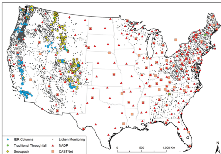
FIG. 2.3 Locations of bulk and through-fall samplers and biomonitoring studies from individual research projects relative to NADP (NTN) and CASTNET national networks. This figure was created by Michael Bell, National Park Service.
