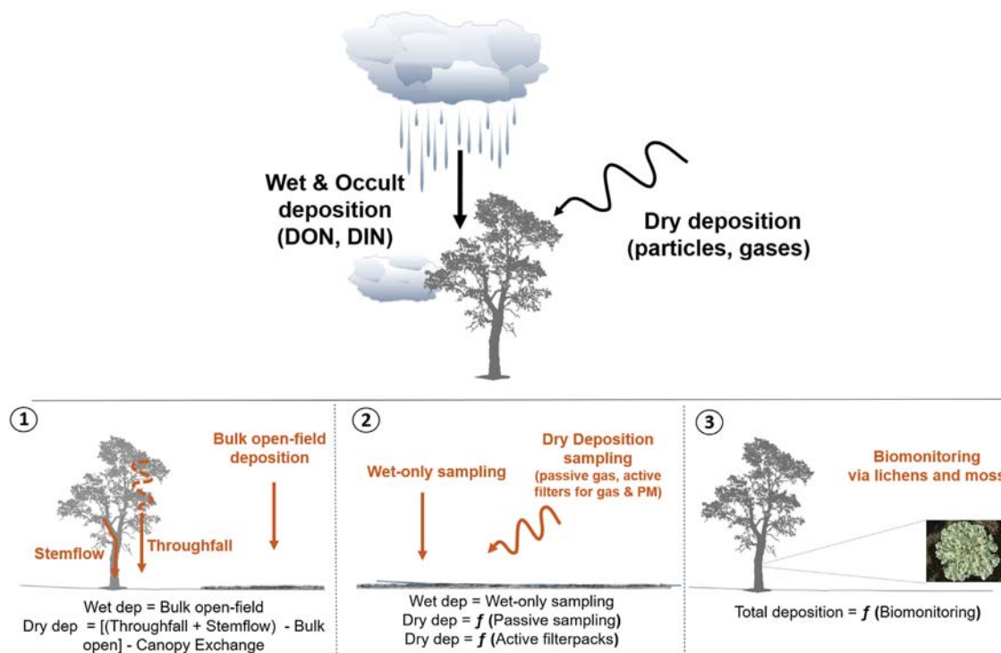
FIG. 2.1 Schematic of deposition processes and N deposition monitoring approaches in forests. A portion of the dry-deposited N will be washed from the canopy in throughfall and stemflow.
