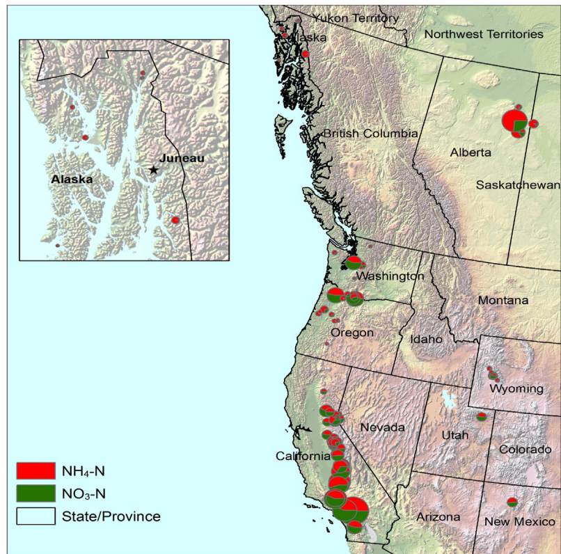
FIG. 2.4 Location of forested sites in western North America where throughfall deposition was measured from 2002 to 2017 using ion exchange resin (IER) samplers. Data are in kg N ha -1 yr -1 (except for the Alaskan sites, which are summertime only). Red portions of the circular symbols represent the proportion of the annual deposition as NH 4 -N and green represents NO 3 -N deposition. The map inset shows details for IER monitoring sites in southeast Alaska, USA. This figure was created by Mark Fenn, USDA Forest Service.
