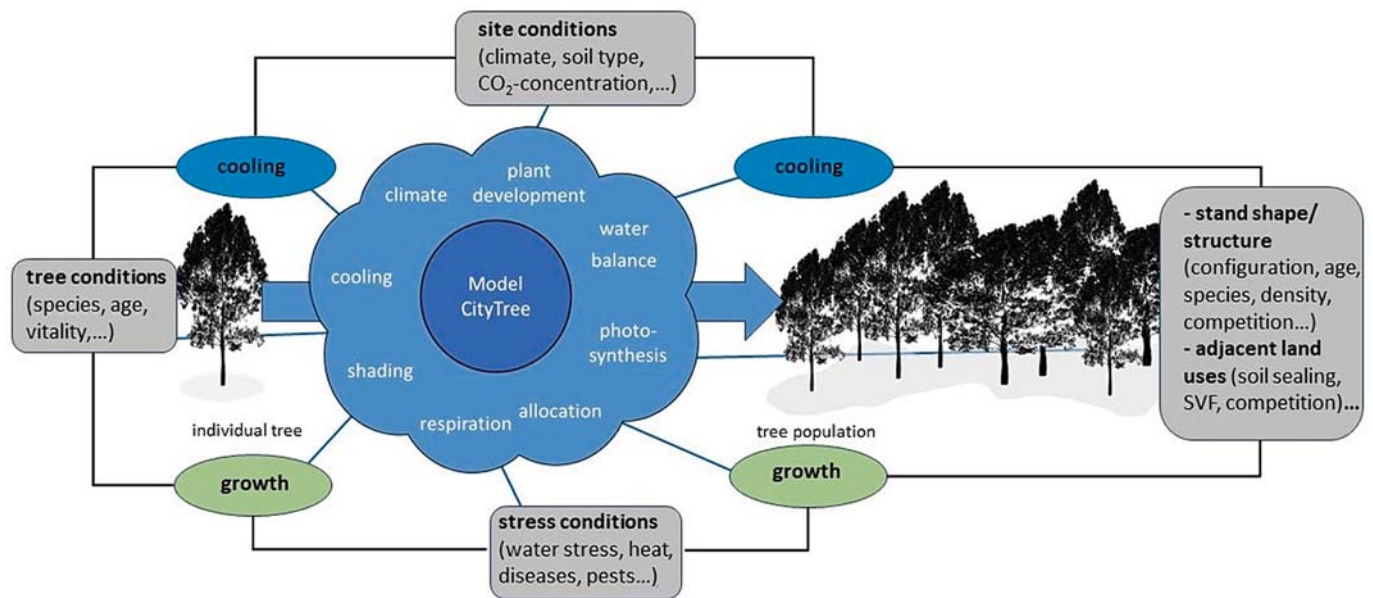
Fig. 6. A proposed schematic diagram of upscaling a process-based tree growth model CityTree (Rötzer et al., 2019) to the plot level.
