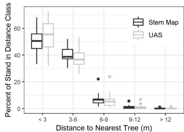
Fig. 8 Boxplots showing the distribution of distance to the nearest tree within the stem-mapped and UAS-extracted tree datasets. The boxplots were developed from the 11 study sites and show the median and interquartile range of distance to the nearest tree within consecutive 3.0-m wide bands
