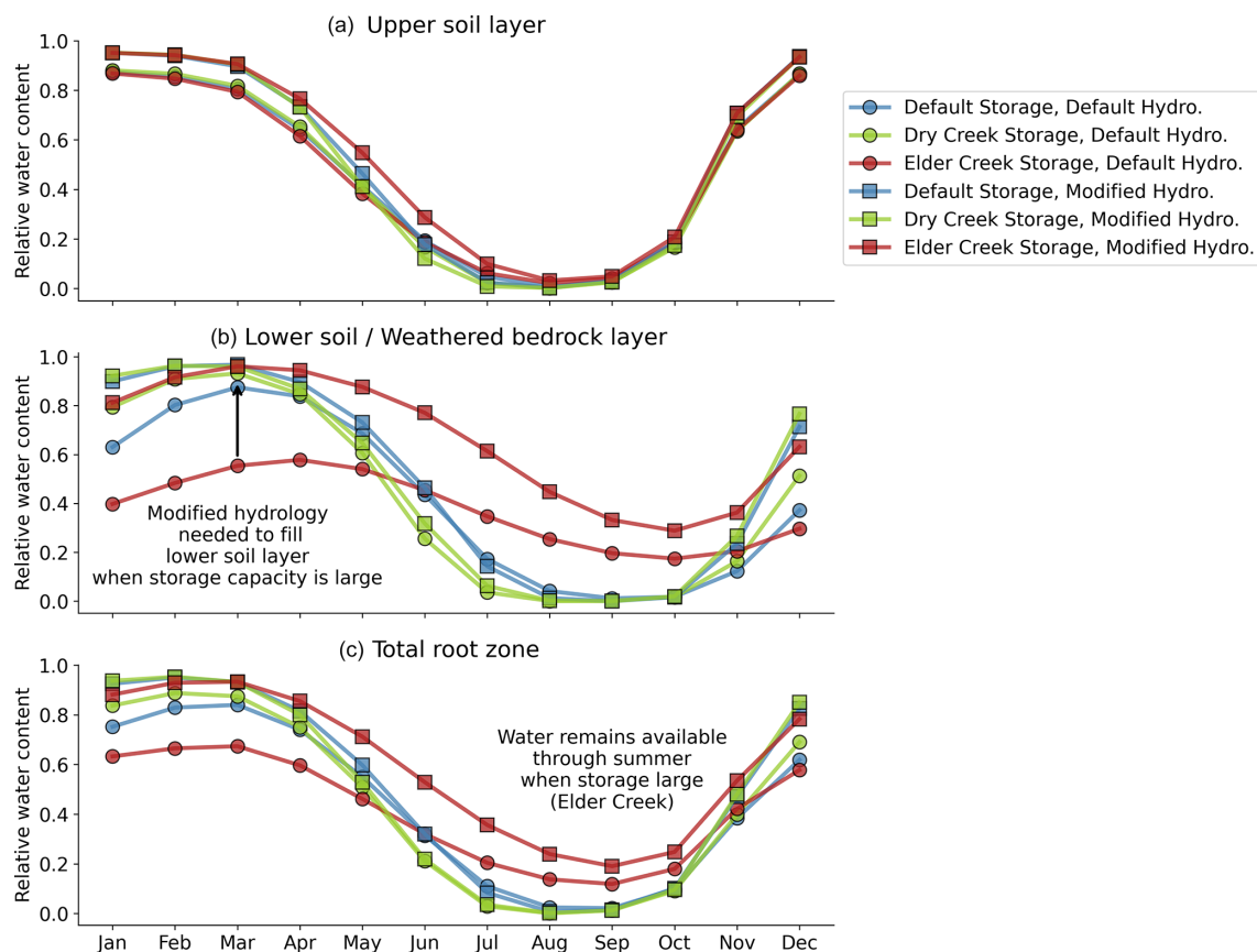
Figure 4. Monthly mean relative water content in the (a) upper soil layer, (b) lower soil or weathered bedrock layer, and (c) total root zone for each model setup. Squares denote the modified hydrology scheme, and circles denote the default hydrology scheme. Color indicates the subsurface storage, with blue default, green Dry Creek, and red Elder Creek. Default and Dry Creek water contents go to zero in the summer for both hydrology schemes. Only the large storage capacity for Elder Creek allows for sustained water supply through the summer. By comparing the circles and squares for each storage, it is clear that more water enters the lower layer with the modified hydrology scheme in the wet season, leading to enhanced water availability even with the same storage.
