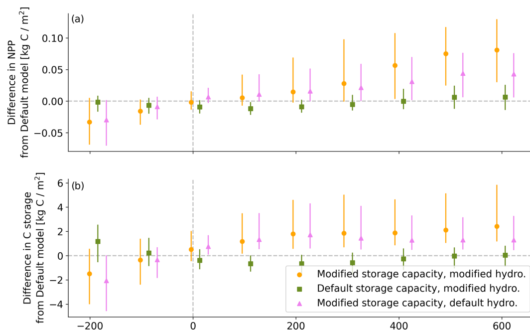
Figure A2. Impact of modified hydrology and storage relative to default LPJ-GUESS model on (a) net primary productivity (NPP) and (b) carbon (C) sequestration. Both NPP and C are enhanced with modified storage and hydrology schemes.
