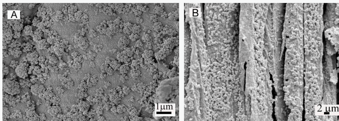
Fig. 2. SEM images of WTHM (A) before and (B) after 960-h exposure to program 1 before and after 960-h exposure to program 1
