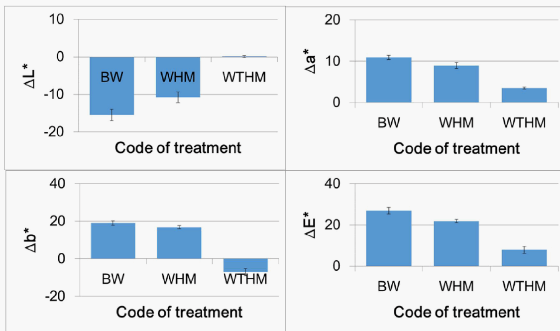
Fig. 4. Surface color changes of wood specimens before and after exposure to UV light for 155 h
