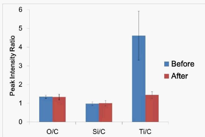
Fig. 3. EDX peak ratios of WTHM before and after 960-h exposure to program 1
