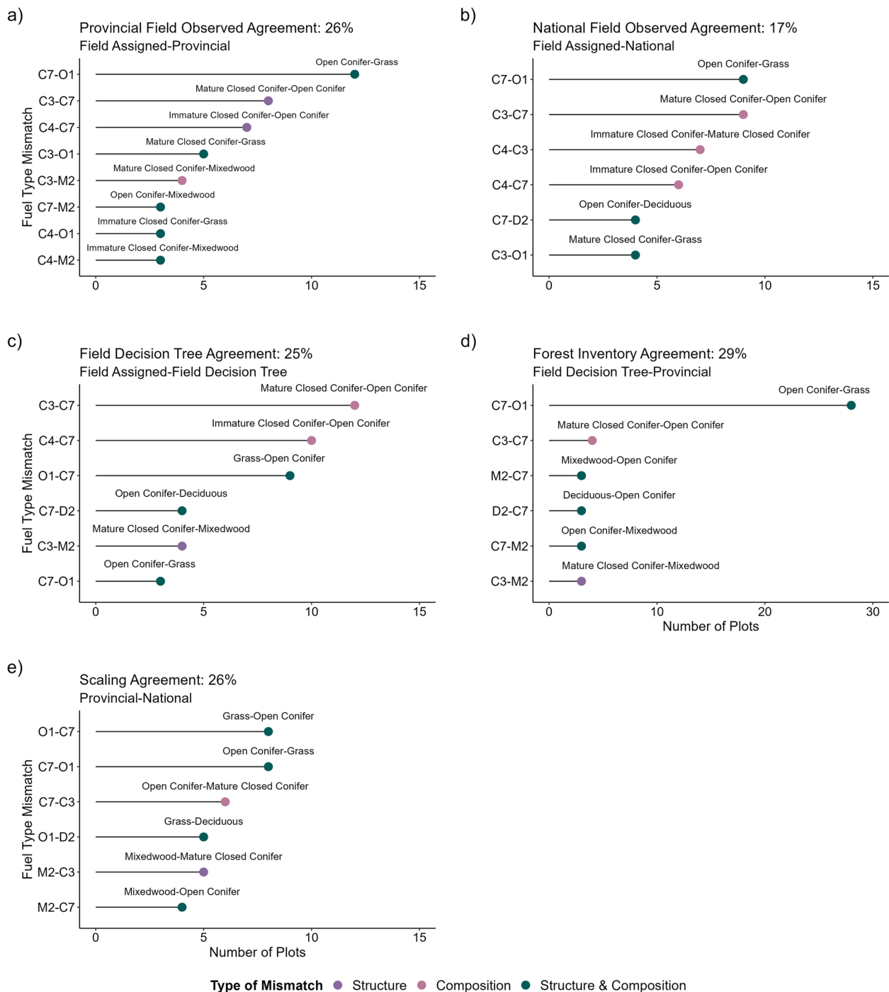
Fig. 4 Frequent ( \geq 3 plots) fuel typing mismatches for a provincial field observed agreement (provincial-field assigned), b national field observed agreement (national-field assigned), c field decision tree agreement (field decision tree-field assigned), d forest inventory agreement (provincial-field decision tree), and e scaling agreement (national-provincial). Labels reflect generalized descriptions of fuel types (e.g., C-3 Mature Jack or Lodgepole Pine is labeled as Mature Closed Conifer). Type of mismatch describes whether the fuel types differ in structure, composition, or structure and composition
