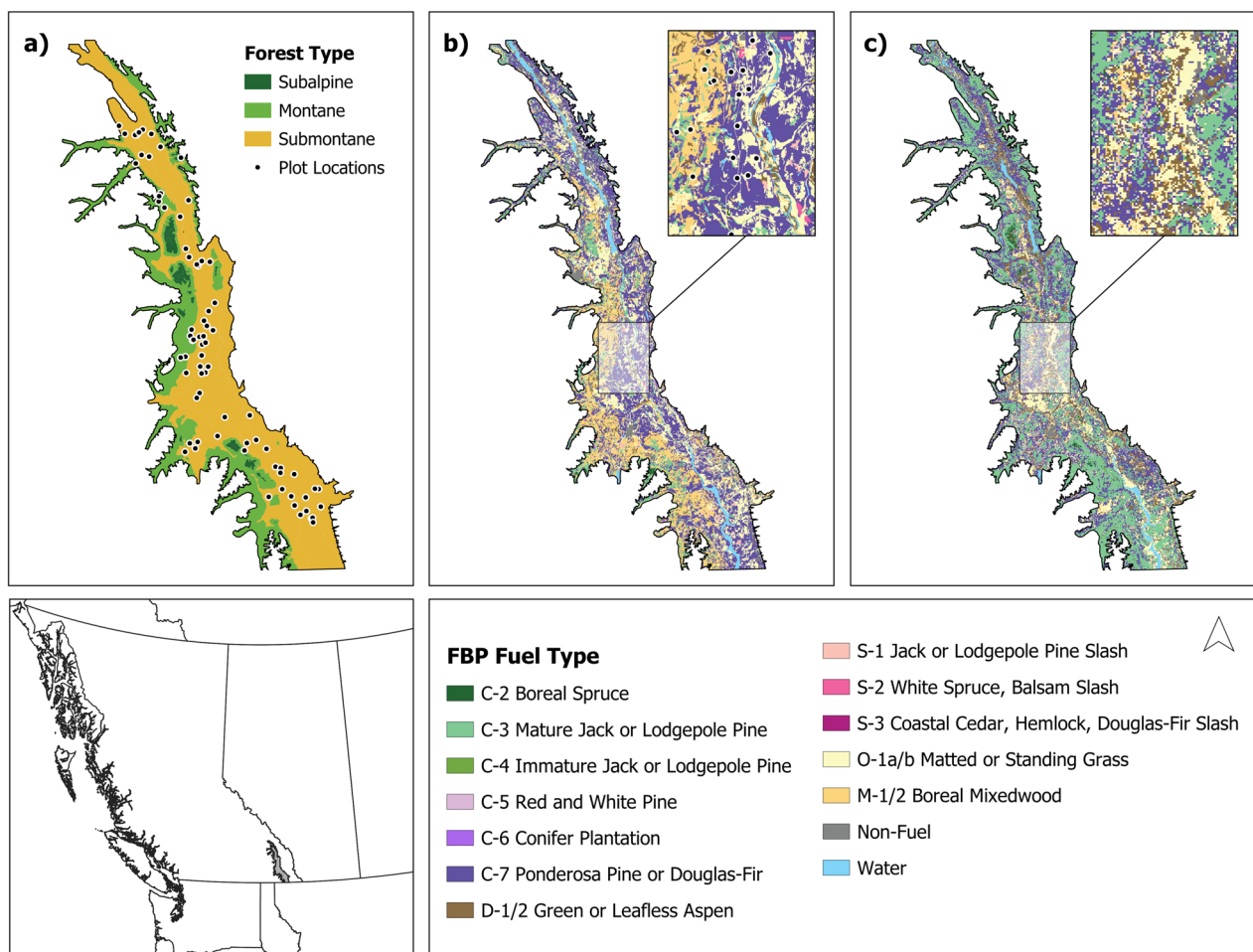
Fig. 1 The southern Rocky Mountain Trench (RMT), located in southeastern British Columbia, Canada, showing a the distribution of forest types and location of field plots ( n=76 ), and Fire Behavior Prediction (FBP) System fuel typing for b 2020 provincial (British Columbia Wildfire Service; 50 m) and c 2019 national (Canadian Forest Service; 250 m) data
