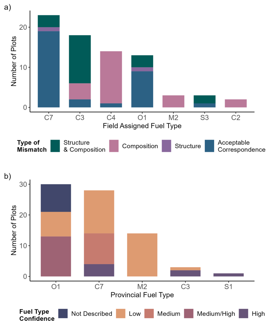
Fig. 3 a Applicability of FBP System fuel types to field plots in interior British Columbia for field assigned fuel types. Applicability is scored as being mismatched to both structure and composition (26.3%, n=20 ), mismatching composition (28.9%, n=22 ), mismatching structure (2.6%, n=2 ), or acceptable correspondence (42.1%, n=32 ). b Fuel type confidence, assigned by BCWS, scored as low (48.7%, n=37 ), medium (13.2%, n=10 ), medium/high (17.1%, n=13 ), high (9.2%, n=7 ), or not described (11.8%, n=9 ) for provincial fuel types
