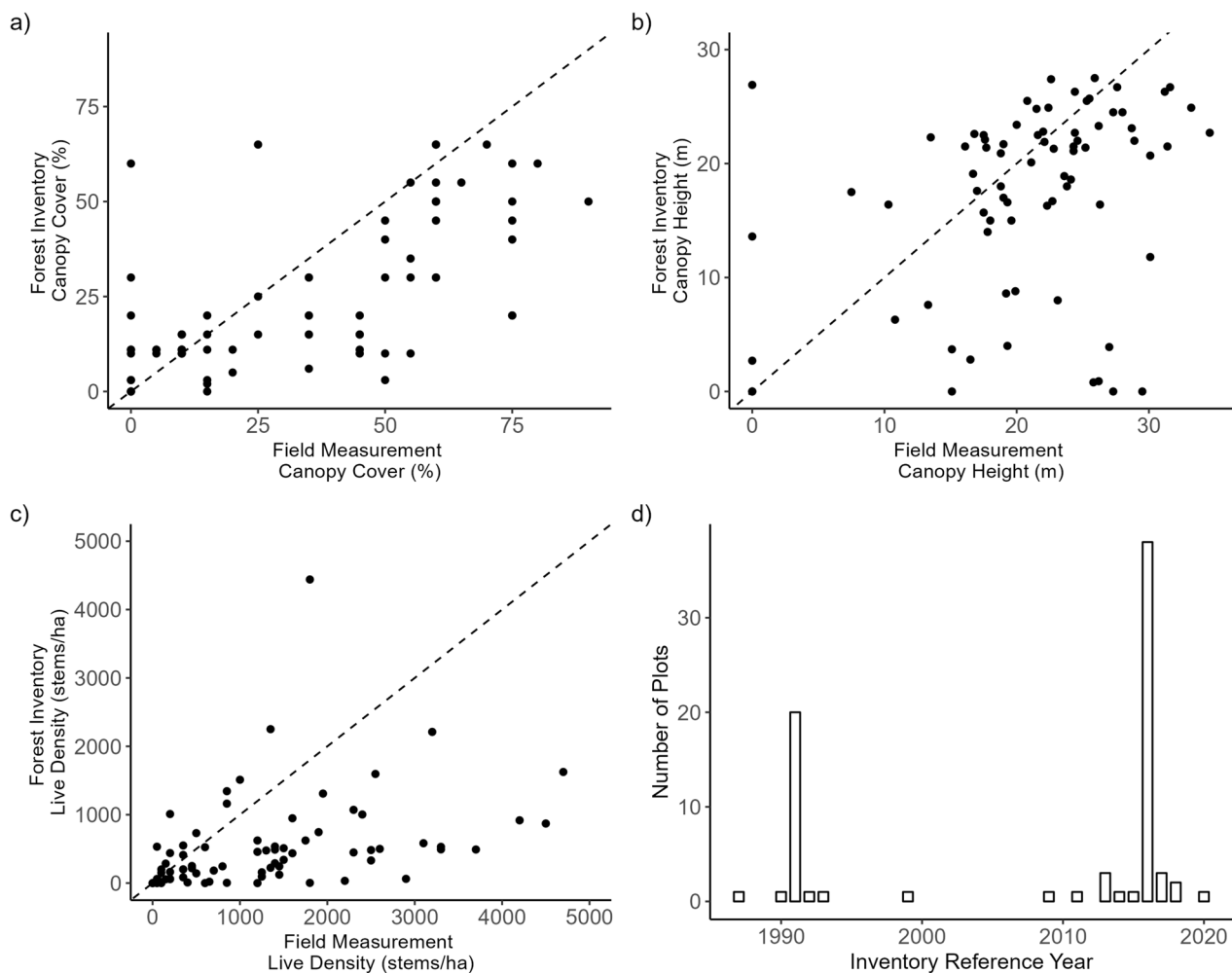
Fig. 5 Agreement between photo-interpreted forest inventory attributes and field measurements of a canopy cover (%), b canopy height (m), and c live density (stems/ha). Dashed lines plot a 1:1 relationship between variables. On average, forest inventory data underpredicts canopy cover by 9.4%, underpredicts canopy height by 3.6 m, and underpredicts live density by 765 stems/ha, relative to field measurements. d Inventory reference year for photo-interpreted forest inventory data
