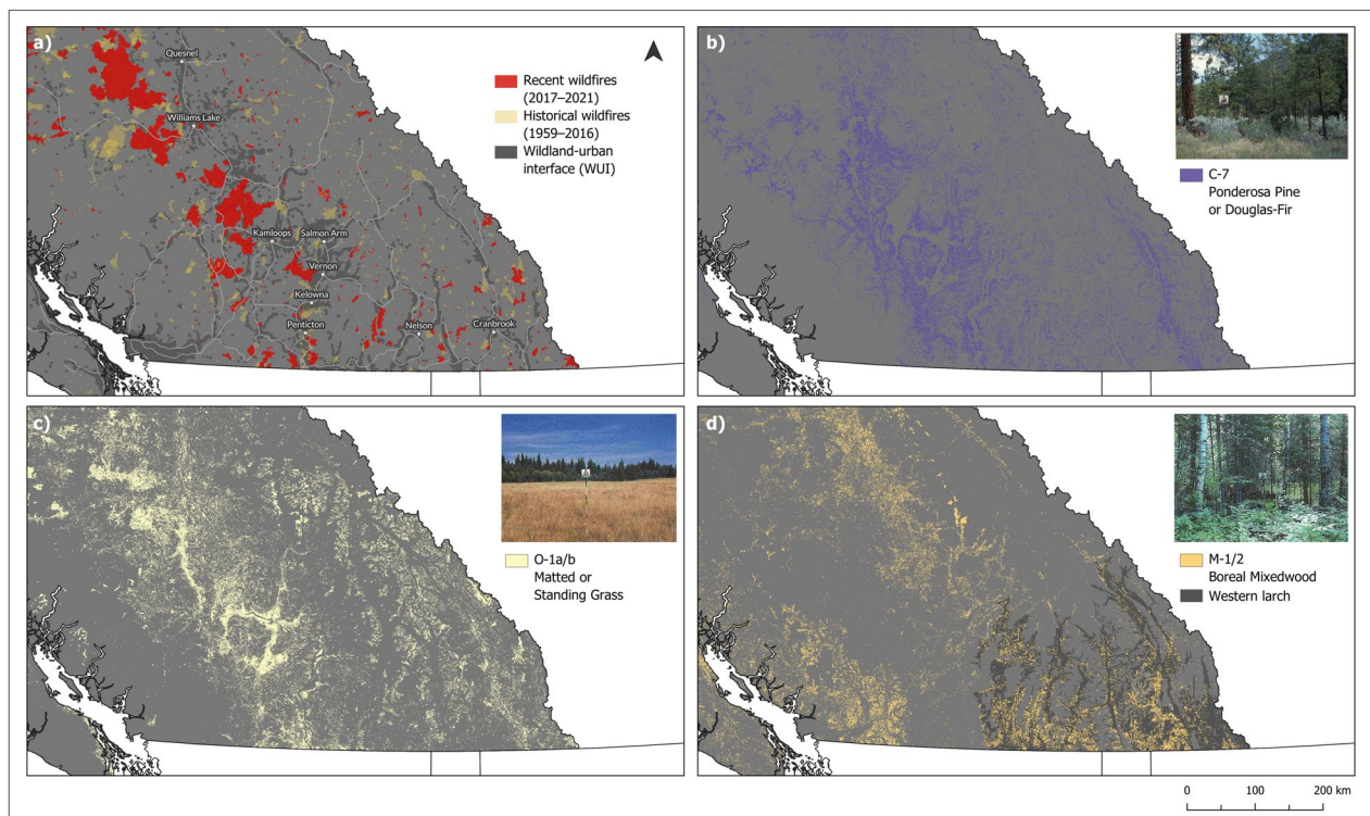
Fig. 6 a Recent (2017–2021) and historical (1959–2016) wildfires (BC Wildfire Service 2023a), the wildland-urban interface (BC Wildfire Service 2023b), and major roads in interior British Columbia. Provincial fuel types with recurring mismatches: b C-7 ponderosa pine or Douglas-fir, c O-1 matted or standing grass, and d M-1/2 boreal mixedwood, with the extent of Western larch (Hamann et al. 2005). Reference Image Source: “FBP Fuel Type Description Webpage ( https://cwfs.cfs.nrcan.gc.ca/background/fueltypes/c1 ).” Canadian Forest Service, Natural Resources Canada. Reproduced with the permission of the Department of Natural Resources, 2023
