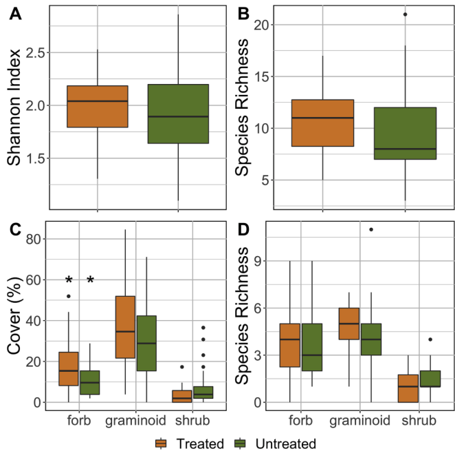
Fig. 8. Box plots showing the range of plot-level values for Shannon Index (A) and species richness (B) for all species, and percent cover (C) and species richness (D) by growth form.
