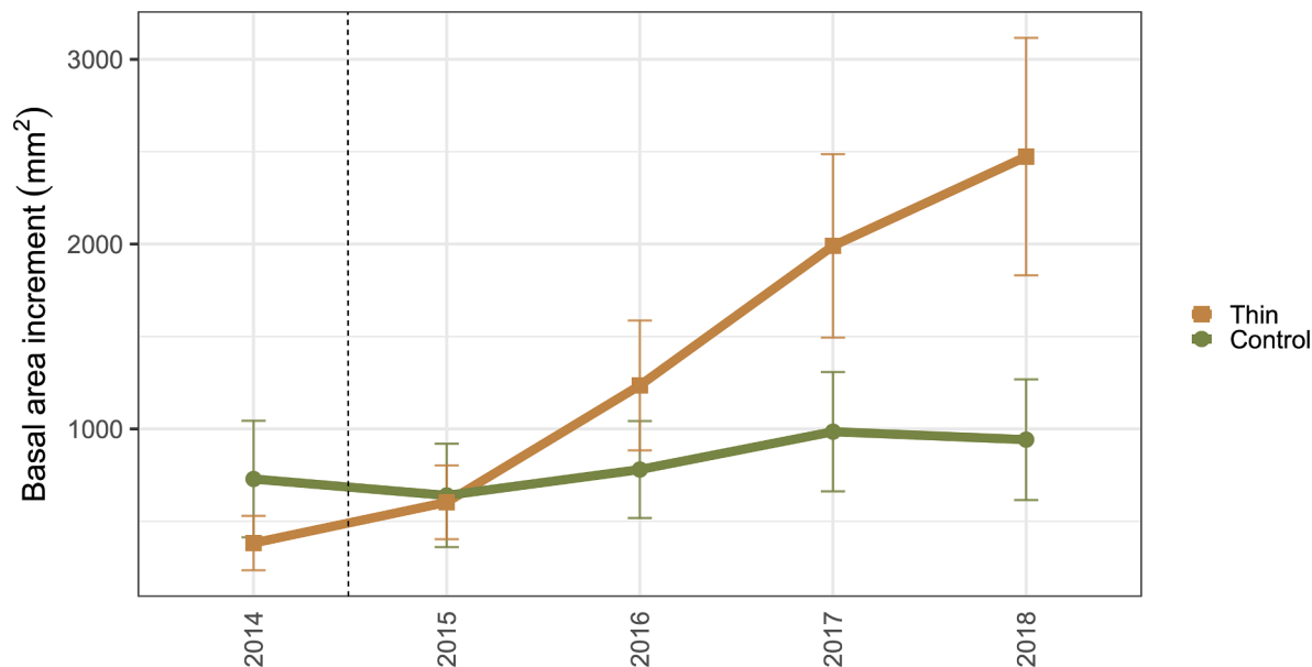
Fig. 3. Estimated mean basal area increment and confidence intervals (whiskers) for treated and untreated stands over the study period (2014–2018). Dashed line represents time of thinning treatment. Results from mixed effects models show that basal area increment was higher in treated stands 3 and 4 years after thinning.
