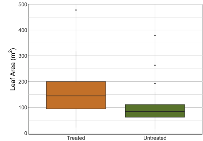
Fig. 6. Box plot of leaf area ( \text{m}^2 ) estimates for trees in treated and untreated stands in 2018 (4 years post-treatment). Results from mixed effects modeling show that thinning increased leaf area, although confidence intervals slightly overlapped zero.
