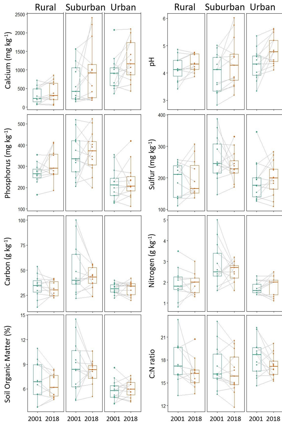
FIGURE 3 | Change in eight soil properties between 2001 and 2018 along the urban-rural gradient. Box plots show changes at the plot level ( n = 36 ) separately for rural (R), suburban (S), and urban (U).
