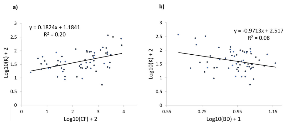
Fig. 2. The relationship between soil infiltration capacity, measured as the unsaturated hydraulic conductivity (K) in cm per hour, and (a) the percent of coarse fragments (CF) in soil and (b) soil bulk density (BD) in 21 forest patches in Baltimore, Maryland, USA.
