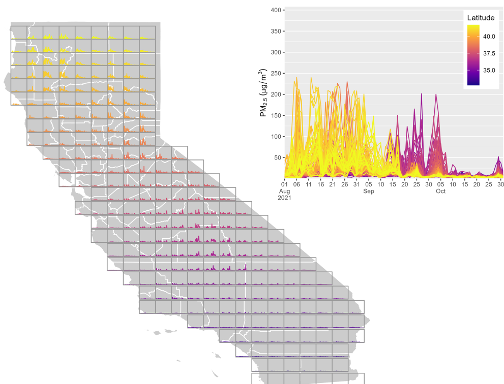
Figure 9. rapidfire \text{PM}_{2.5} estimates for August–October 2021. Each box on the map shows the time series for a point at the centroid of the box, and the larger plot shows all of those time series overlaid.
