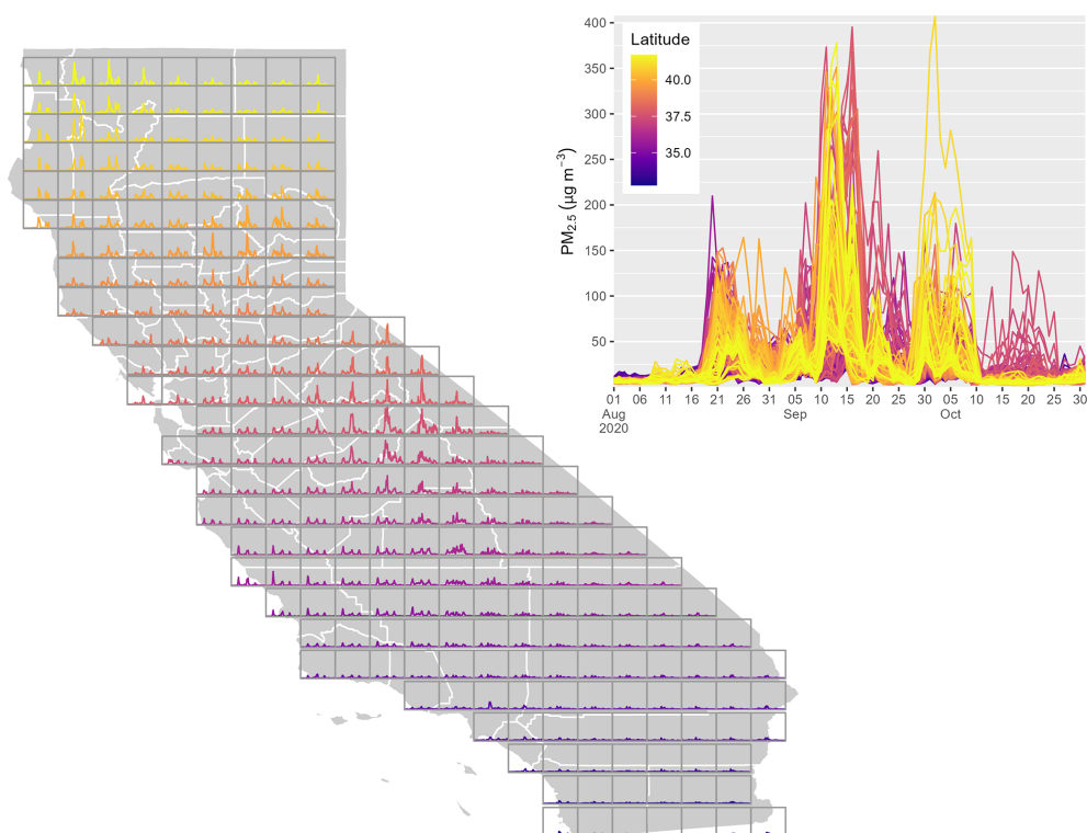
Figure 8. rapidfire \text{PM}_{2.5} estimates for August–October 2020. Each box on the map shows the time series for a point at the centroid of the box, and the larger plot shows all of those time series overlaid.
