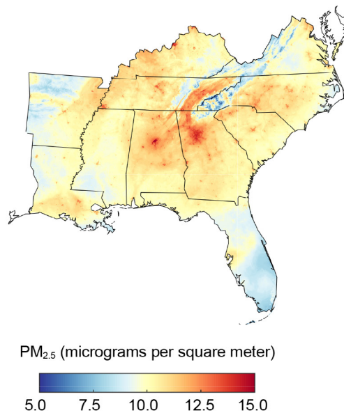
a) Present-day (2000–2019) average PM 2.5 levels
