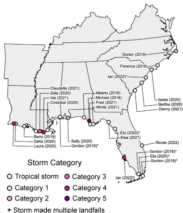
b) Southeast Hurricane Landfalls (2018–2022)
