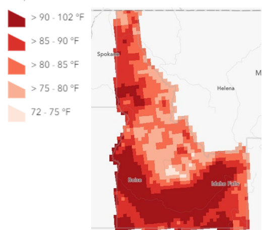
RCP 8.5 End-Century: Summer Max Daily Temperature
