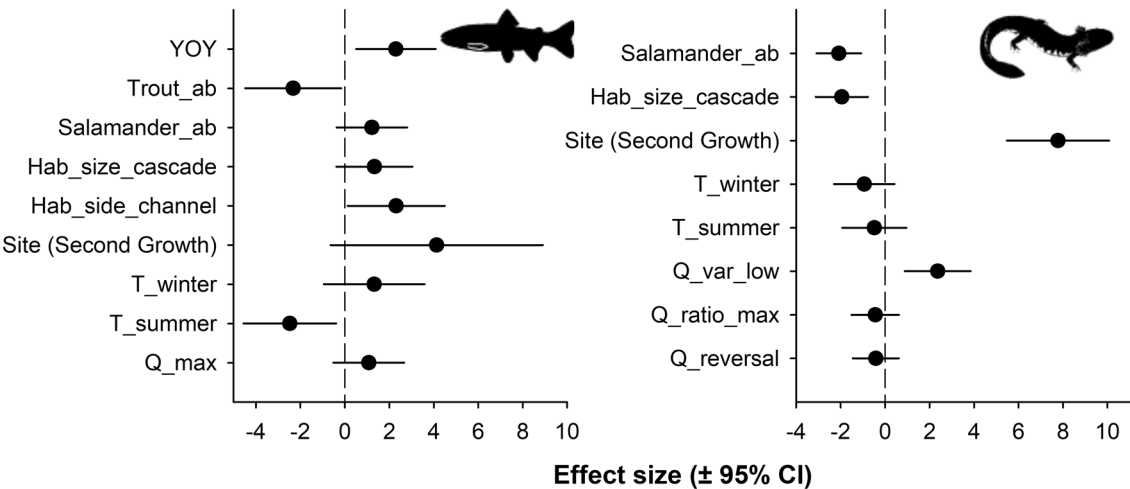
Figure 6. Effect size (standardized values ± 95% CI) of covariate factors from the best-supported model (Tables 3, 4; Tables S10, S11) explaining median size of adult Coastal Cutthroat Trout and Coastal Giant Salamanders in Mack Creek. The best-supported model included both density-dependent (abundance of animals) and density-independent (stream discharge, temperature, habitat size) factors. These biotic and abiotic factors are fully described in Table 1.
