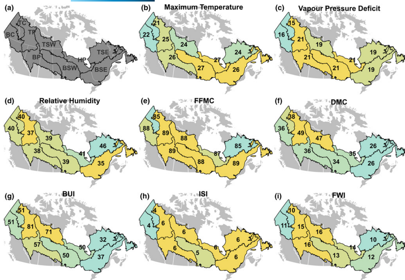
FIGURE 4 Thresholds for reburning weather days within (a) Canadian boreal forest ecozones. Ecozones displayed are the Taiga Cordillera (TC), Boreal Cordillera (BC), Taiga Plains (TP), Boreal Plains (BP), Taiga Shield West (TSW), Boreal Shield West (BSW), Hudson Plains (HP), Taiga Shield East (TSE), and Boreal Shield East (BSE). Weather variables displayed are: (b) maximum temperature ( ^{\circ}\text{C} ), (c) vapour pressure deficit (hPa), (d) relative humidity (%), (e) Fine Fuel Moisture Code (FFMC), (f) Duff Moisture Code (DMC), (g) Buildup Index (BUI), (h) Initial Spread Index (ISI) and (i) Fire Weather Index (FWI). Colours correspond to the weather threshold values, with blue indicating a lower threshold and yellow indicating a higher threshold relative to fire weather severity.
