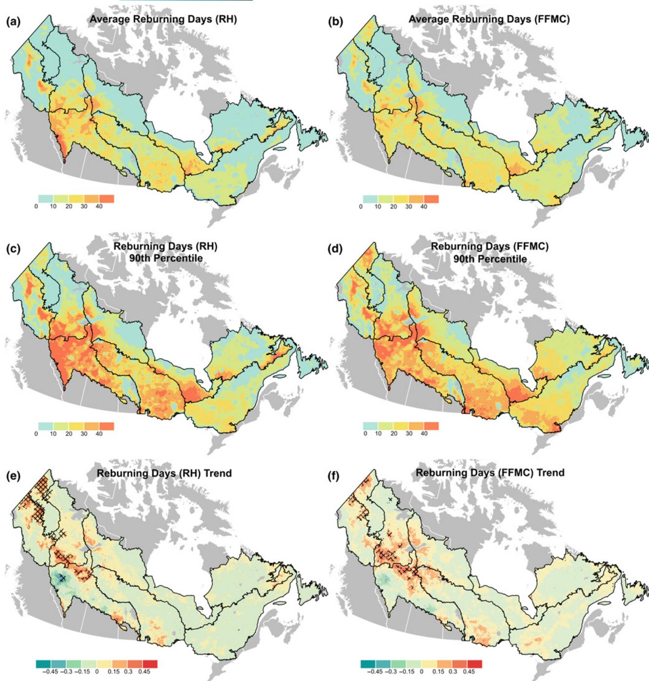
FIGURE 5 Average (a, b) number of reburning weather days in a fire season, 90th percentile (c, d) number of reburning weather days in a fire season and trends (e, f) in the annual number of reburning weather days (1981–2021). Days with extreme weather conducive to reburning were identified using Relative Humidity (RH; a, c, e) and Fine Fuel Moisture Code (FFMC; b, d, f) reburning weather thresholds. Trends are represented by Sen's slopes, with areas of significant trends overlaid with black hash marks.
