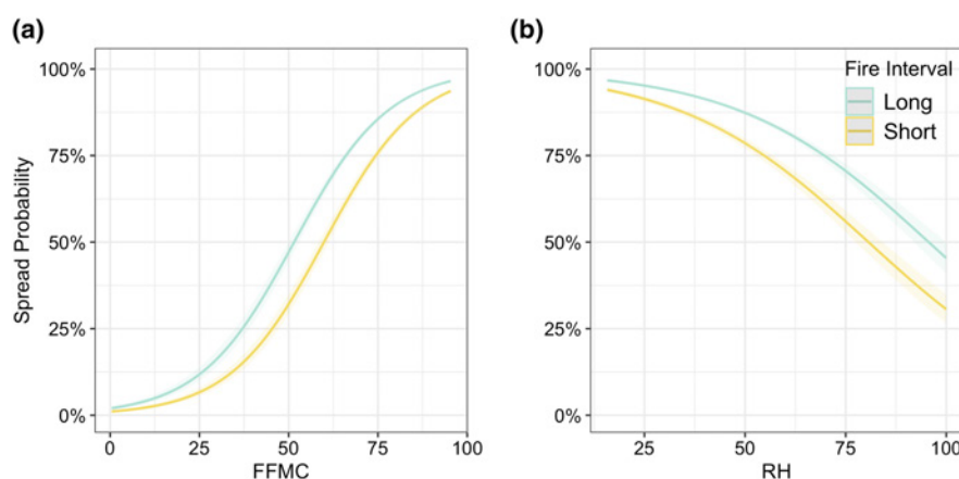
FIGURE 1 Marginal effect plots of the probability of short- and long-interval fire spread, as a function of daily fire weather (a) Fine Fuel Moisture Code (FFMC), and (b) relative humidity (RH; %) in a logistic generalized linear mixed-effect model, with short-interval fire spread defined as \leq 20 years between fires (Equation 1; Table 2).
