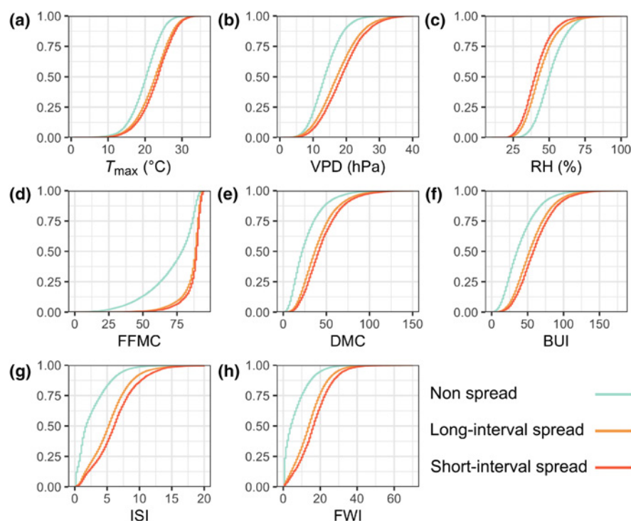
FIGURE 2 Empirical cumulative distribution functions of daily weather during short- and long-interval fire spread and non-spread days. Weather variables shown are (a) maximum temperature ( T_{\text{max}} ), (b) vapour pressure deficit (VPD), (c) relative humidity (RH), (d) Fine Fuel Moisture Code (FFMC), (e) Duff Moisture Code (DMC), (f) Buildup Index (BUI), (g) Initial Spread Index (ISI) and (h) Fire Weather Index (FWI).
