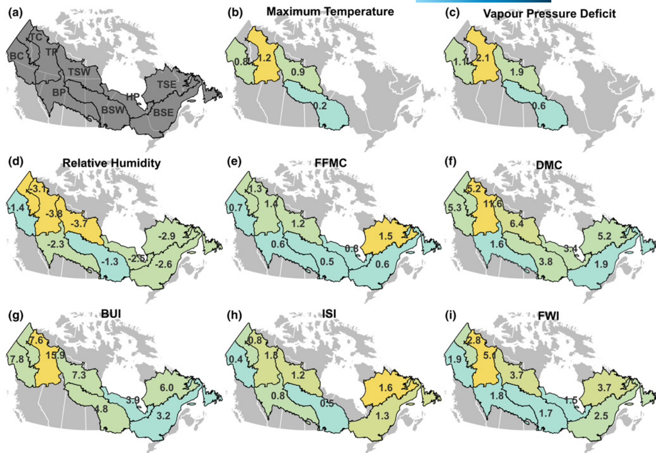
FIGURE 3 Medians of differences between short- and long-interval spread day fire weather within (a) Canadian boreal forest ecozones. Ecozones displayed are the Taiga Cordillera (TC), Boreal Cordillera (BC), Taiga Plains (TP), Boreal Plains (BP), Taiga Shield West (TSW), Boreal Shield West (BSW), Hudson Plains (HP), Taiga Shield East (TSE), and Boreal Shield East (BSE). Weather variables displayed are: (b) maximum temperature ( ^{\circ}\text{C} ), (c) vapour pressure deficit (hPa), (d) relative humidity (%), (e) Fine Fuel Moisture Code (FFMC), (f) Duff Moisture Code (DMC), (g) Buildup Index (BUI), (h) Initial Spread Index (ISI), and (i) Fire Weather Index (FWI). Ecozones displayed have significant differences in daily weather between short- and long-interval fire spread days. Colours correspond to the difference in weather conditions between short- and long-interval spread days, with blue indicating a smaller difference and yellow indicating a greater difference.
